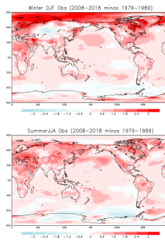
Figure 1. Polar Amplification using Long-term observations of Surface Air Temperatures ( ^{\circ}\text{C} ) at 2008-2018 (seasonal average) relative to 1979-1989 (seasonal average) in (a) Winter (DJF) and (b) Summer (JJA). Source: Era Interim Reanalysis.
