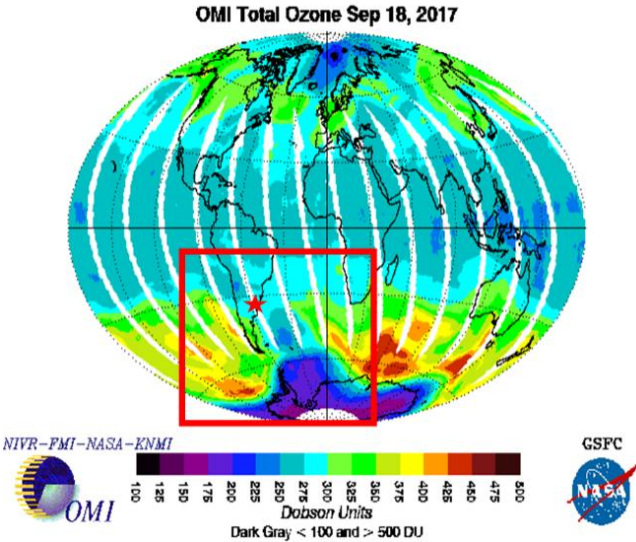
Figure 2: a) Retroactive trajectories as retrieved by model LagrangianHYSPLIT model, initialized on 09/19/17 00UTC at SSO location. The back-trajectories were run at 20 km (in red), 24 km (in blue) and 28 km (in green) above ground level; b) global TOC distribution as recorded by OMI experiment on 18 SEPT. 2017. The red box focus on the low-ozone event and the stare symbol indicates the location of the SSO site.
