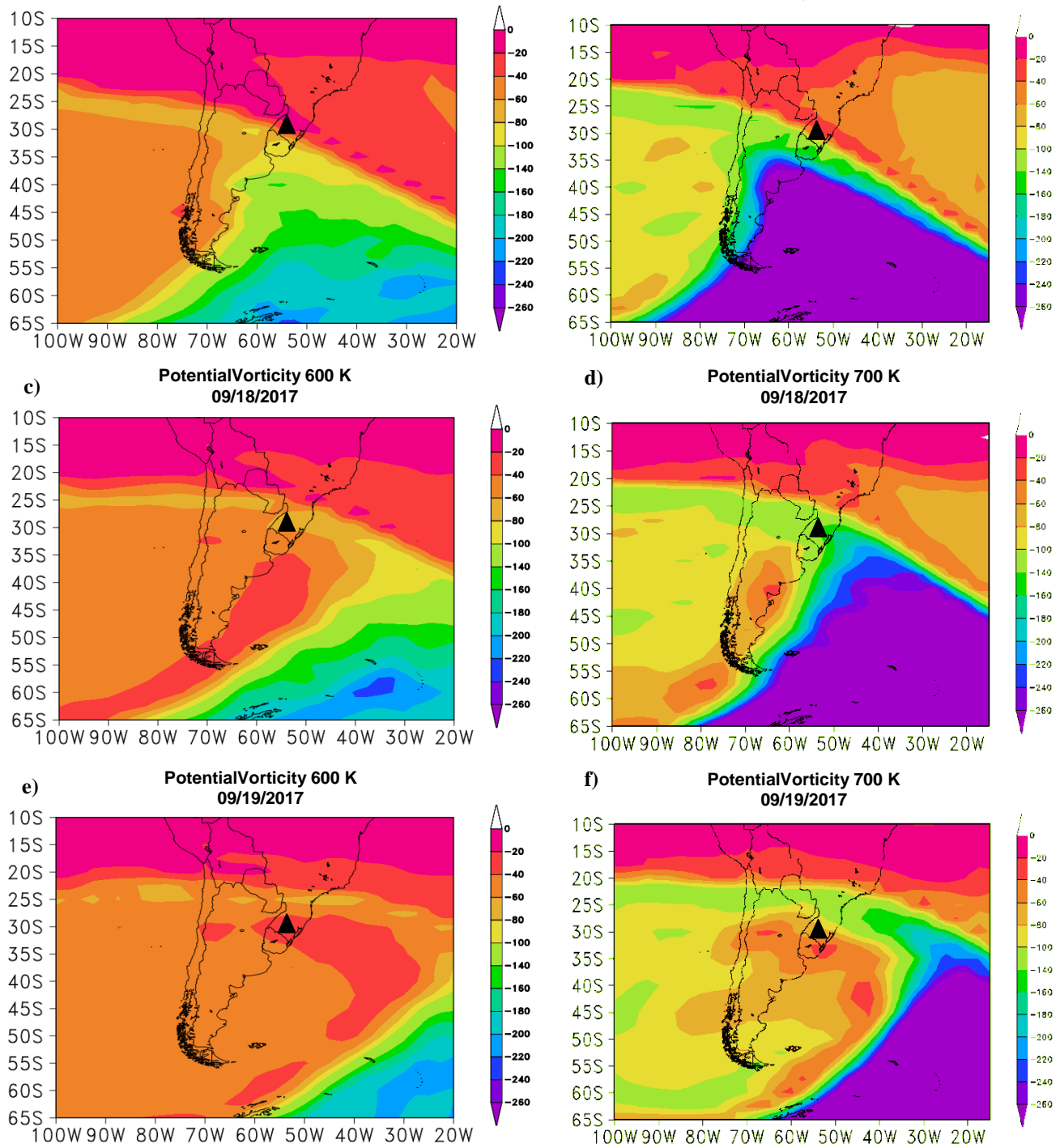
Figure 1: Potential Vorticity fields at the 600 K and 700 K isentropic level as derived from ECMWF data successively on (a) and (b) 17 SEPT., (c) and (d) 18 SEPT., and (e) and (f) 19 SEPT. 2017. The black symbol indicates the location of the SSO.
