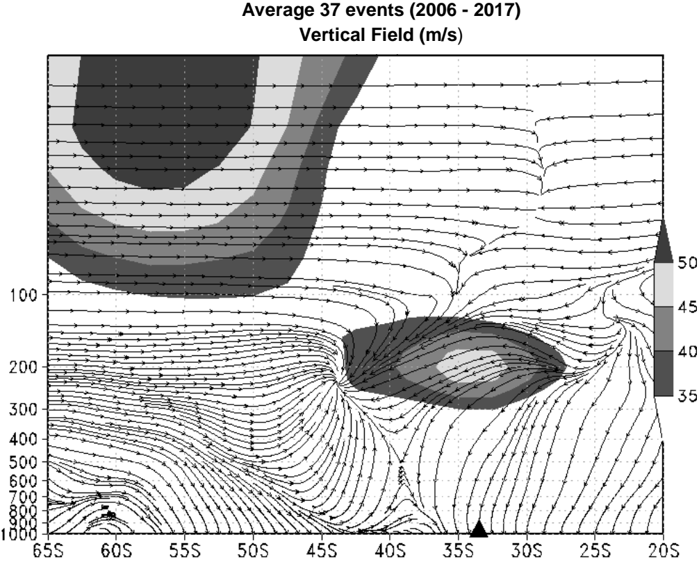
Figure 7: Average for the 37 events of the vertical field between 1000 and 30 hPa, showing the jet current (shaded gray) in m/s.
