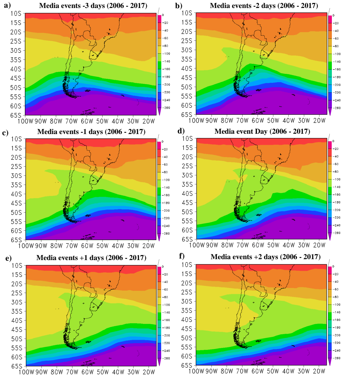
575 Figure 4: Average PV maps at the 700K isentropic level from 37 PV distributions detected as secondary effect events of AOH: a) -3 days, b) -2 days, c) -1 day, d) day of the event, e) +1 day, f) +2 days.
