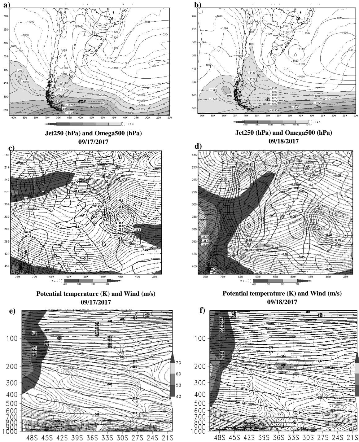
Figure 3: Pressure fields at medium sea level, horizontal cut of the atmosphere and vertical cut between 1000 and 50hPa for days a), c) and e) 09/17/2017 and b), d) and f) 09/18/2017. The red symbol indicates the location of the SSO site.
