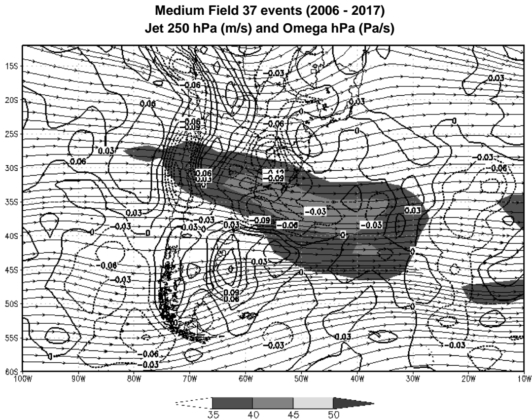
Figure 6: Mean field for the 37 AOH side effect events in the analysis period with jet at 250 hPa (shaded) and Omega at 500 hPa (Omega positive solid lines, Omega negative dotted lines).
