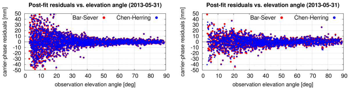
10 Figure 7. Post-fit phase residuals distribution when using different gradient mapping functions, Bar-Sever (red) and Chen and Herring (blue), and observation weighting: SINEL2 (left) and EQUAL (right).
