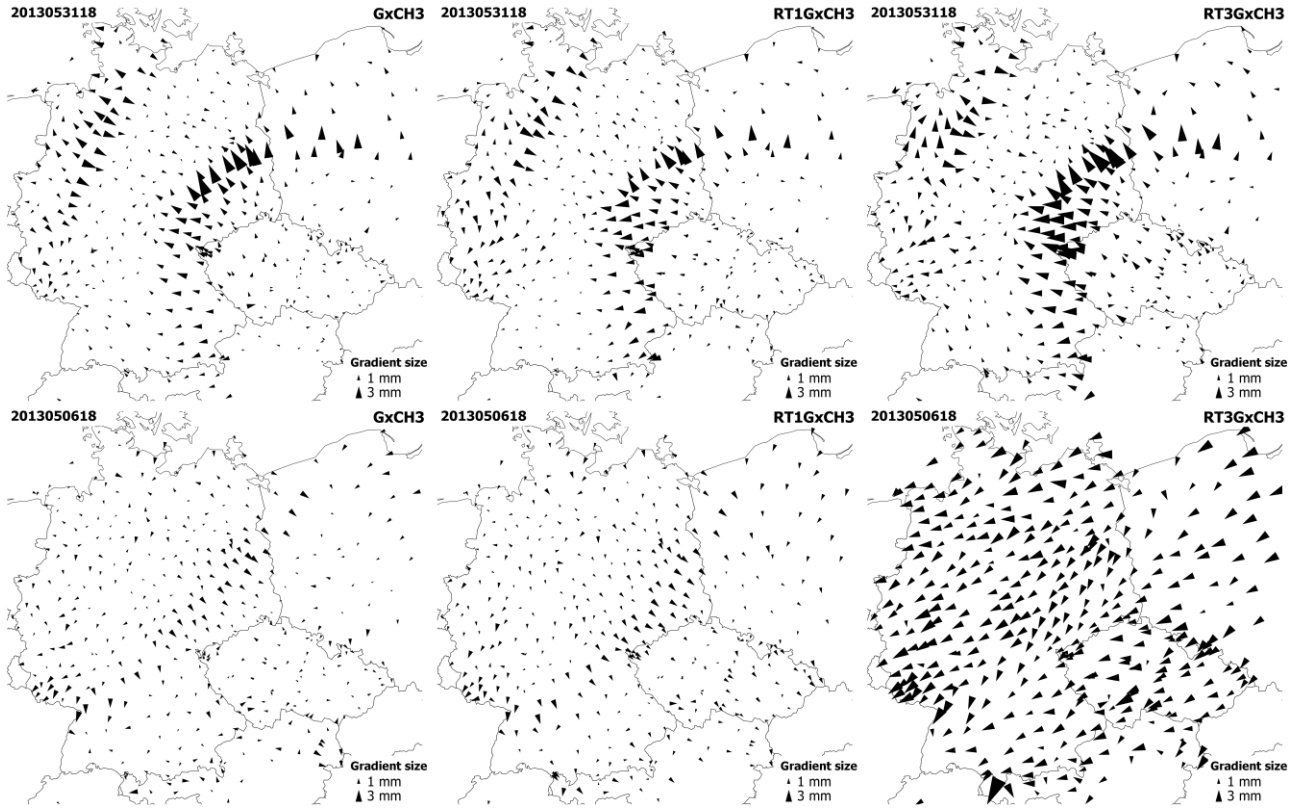
Figure 34. Tropospheric gradient maps from GNSS GxCH3 solution (left), GNSS RT1GxCH3 solution (middle) and GNSS RT3GxCH3 solution (right) on 31 May 2013, 18:00 UTC (top) and on 06 May 2013, 18:00 UTC (bottom).
