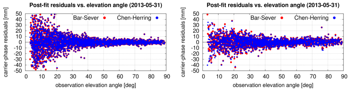
Figure 67. Post-fit phase residuals distribution when using different gradient mapping functions, Bar-Sever (red) and Chen and Herring (blue), and observation weighting: SINEL2 (left) and EQUAL (right).
