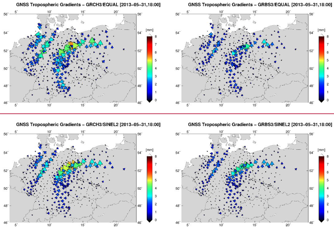
Figure 4. Tropospheric gradient maps on May 31, 2013 (18:00 UTC) from GNSS solutions using: Chen and Herring mfg (left), Bar-Sever mfg (right) and EQUAL (top) and SINEL2 (bottom) observation weighting schemes.
