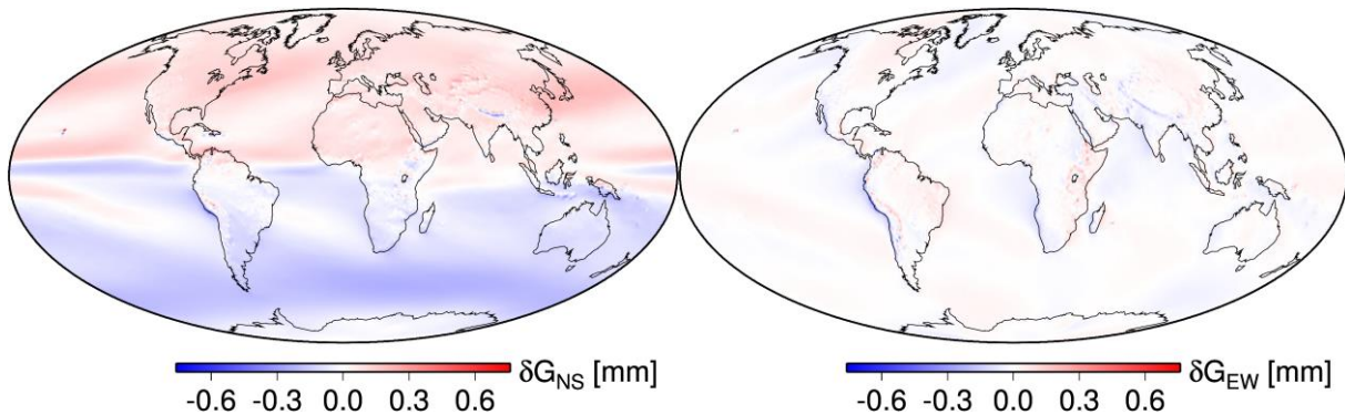
Figure 7.8. Systematic difference (average over 10 years) for any point on Earth's surface between tropospheric gradients estimated utilizing the gradient mapping function of Bar-Sever and tropospheric gradients estimated utilizing the gradient mapping function of Chen and Herring. The left panel shows the north gradient component, the right panel the east gradient component. The result is based on ERA5 data.
