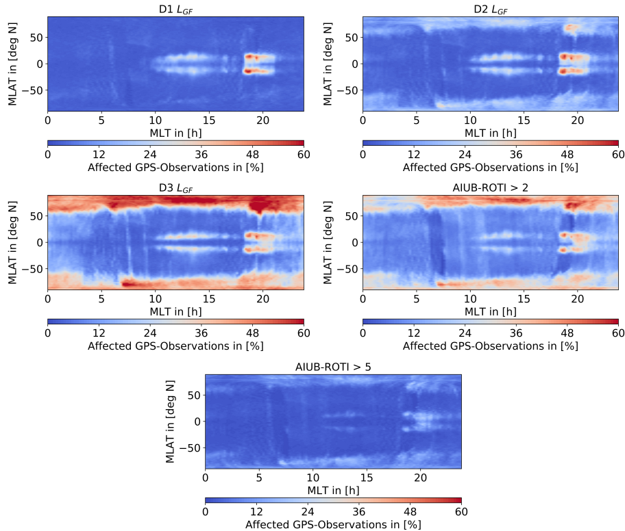
Figure 10. Ammount of weighted raw GPS measurements for the analyzed test period,2015: Jan., Mar.; 2016: Feb., Mar., Jun., Jul., Aug., binned to the corresponding LEO position. Top: D1- L_{GF} (left), D2- L_{GF} (right), middle: D3- L_{GF} (left), ROTI>2 (right), bottom: ROTI>5. Binsize 1^\circ Mlat \times 0.2 h MLT
