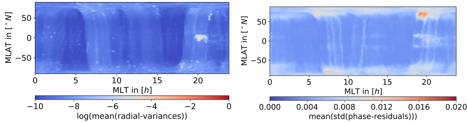
Figure 3. Radial variances (left) and spreading of phase residuals (right) binned in magnetic coordinates for the analyzed test period, 2015: Jan., Mar.; 2016: Feb., Mar., Jun., Jul., Aug.
