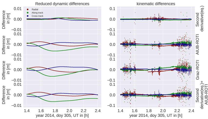
Figure 12. Differences between the unweighted positions of reduced-dynamic (left) and kinematic (right) orbits. All orbits were compared to the unweighted case. The second derivative-based weighting was limited to the equatorial region (eq.)
