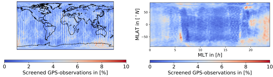
Figure 5. Average number of GPS-observations screened in the preprocessing for the analyzed test period, 2015: Jan., Mar.; 2016: Feb., Mar., Jun., Jul., Aug.. Left: geographic coordinates, right: magnetic coordinates
