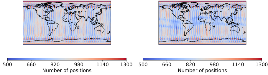
Figure 13. Number of kinematic positions for the analyzed test period, 2015: Jan., Mar.; 2016: Feb., Mar., Jun., Jul., Aug., un-screened (left) and with AIUB standard screening (right). Binned in 1^\circ \times 1^\circ grid.
