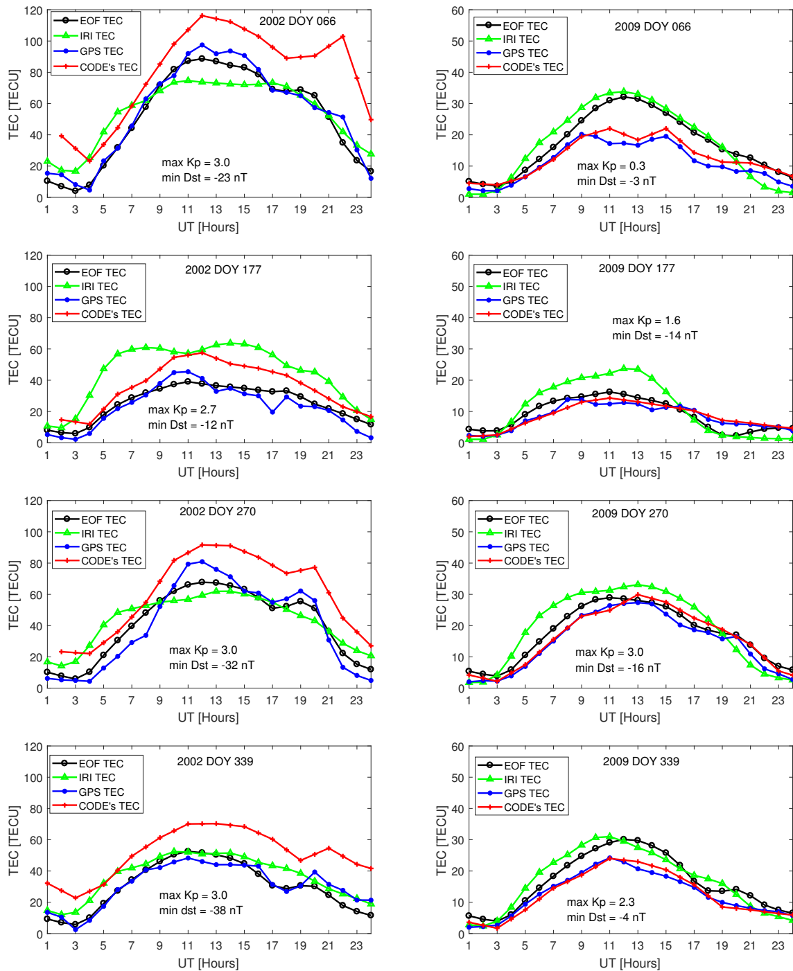
Figure 3. GPS TEC, IRI TEC, CODE's TEC and the EOF TEC over Malindi for some selected max quiet days. Included in each plot are the maximum Kp and the minimum Dst index for the day.
