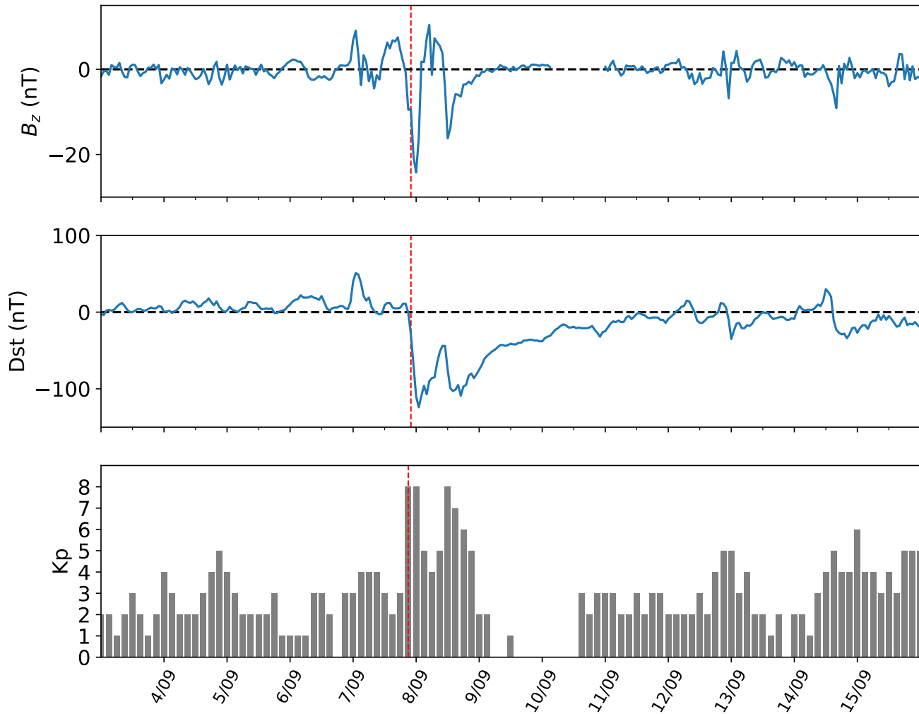
Figure 1. The vertical component of interplanetary magnetic field ( B_z ) and the Dst and Kp indices between September 3 and September 16, 2017. The vertical red dashed line in all the plots points to the storm sudden commencement.
