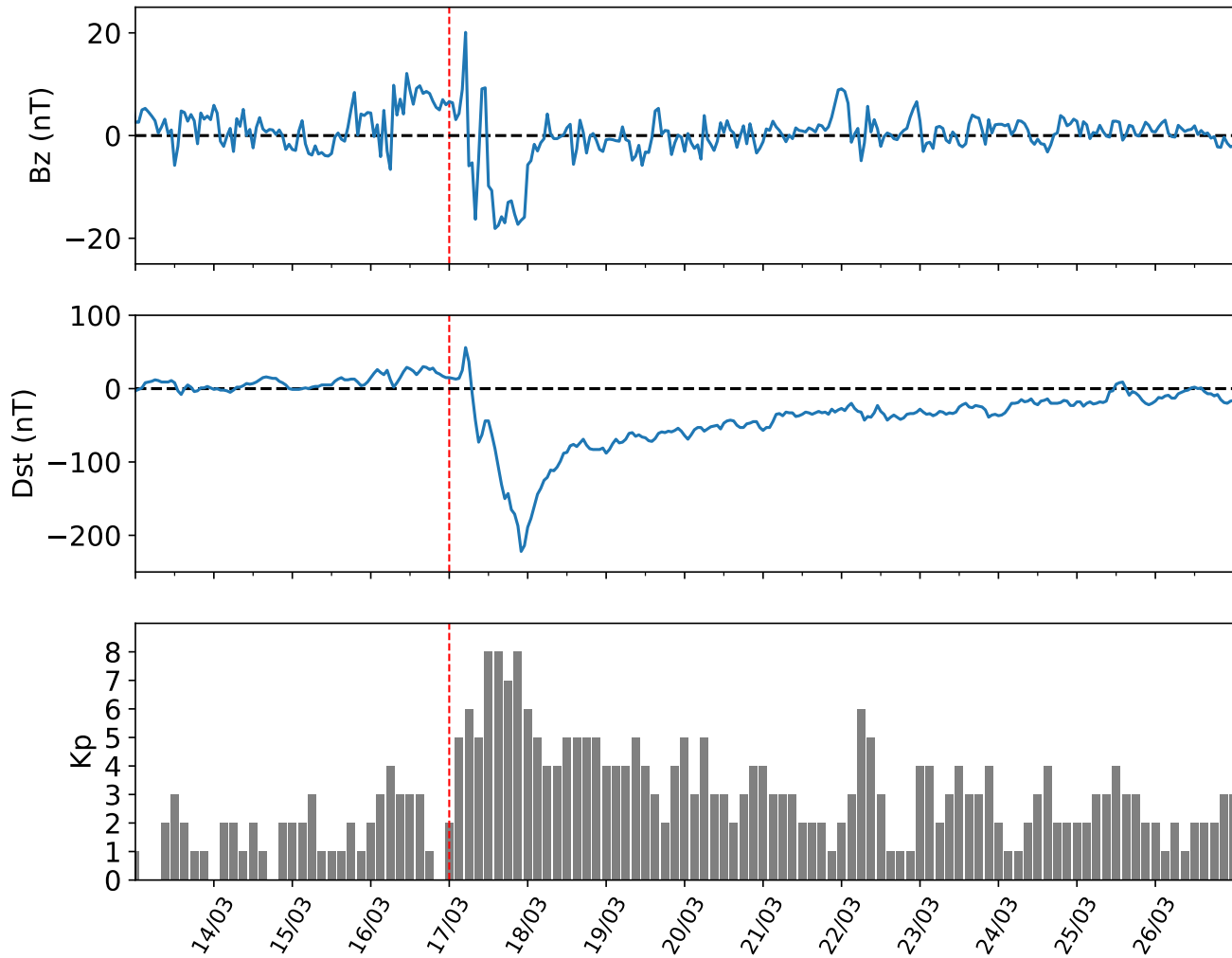
Figure 5. The vertical component of the interplanetary magnetic field ( B_z ) and the Dst and Kp geomagnetic indices between March 13 and March 27, 2015. The vertical red dashed line in all the plots indicates the day that the 2015 St. Patrick's day storm occurred (March 17, 2015).
