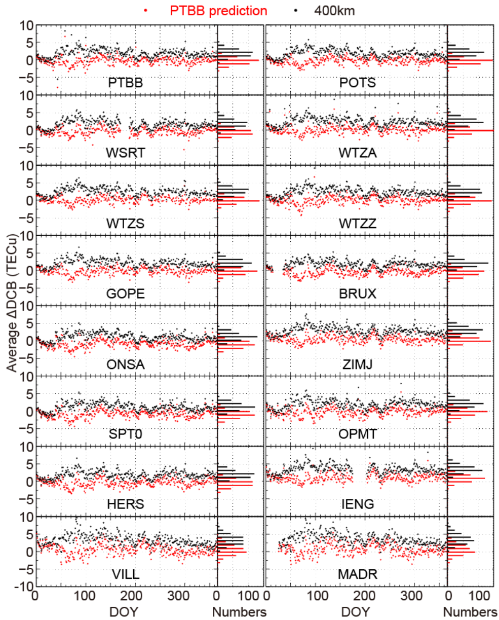
Fig.5 Comparisons of the average \Delta DCB calculated using the predicted optimal ionospheric shell heights (red dots) and those using the fixed ionospheric shell height (black dots) in 2014 for stations in Region II.
