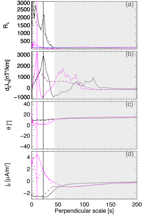
Figure 6. Sections in the MSMVA spectra scalograms showing the dependence of the parameters as a function of the perpendicular scale (scale corrected). a) R_\lambda ; b) \partial_\xi \lambda_\eta ; c) \theta ; d) j_{||} . Solid/dashed lines indicate the profiles for the linear/logarithmic scale sampling scheme. The profiles are taken in the middle of the upward and downward FACs located at 03:24:43 and 03:25:00, respectively. These times are indicated by the vertical solid lines in Figure 5 (same color code). The vertical black/magenta lines indicate the scales of these FAC elements as identified by \partial_\xi \lambda_\eta . The horizontal blue line in (a) indicates a reference level, R_\lambda=100 , discussed in the text. The marked gray area indicates the region where R_\lambda < 100 for the selected sections.
