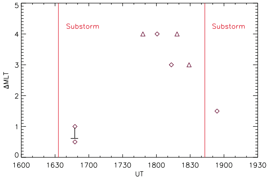
Figure 10. Time evolution of asymmetric conjugate auroral features. Diamonds are auroral asymmetries identified from Figure 3 and 4, while triangles are identified from images not shown, but can be found in auxiliary material. The red vertical lines are the times of the substorms.
