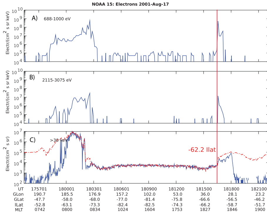
Figure 6. Particle measurements from NOAA 15 pass in the southern hemisphere on August 17, 2001, see trajectory in Figure 4C. It passed through the dusk-side aurora at 18:17 UT. A) Electron flux: 688-1000 eV. B) Electron flux: 2115-3075 eV. C) Electron flux: \geq 30 keV, where blue line shows electrons within the loss cone and red line shows the locally mirroring electrons. Red vertical line shows the poleward edge of precipitation at -62.2^\circ magnetic latitude.
