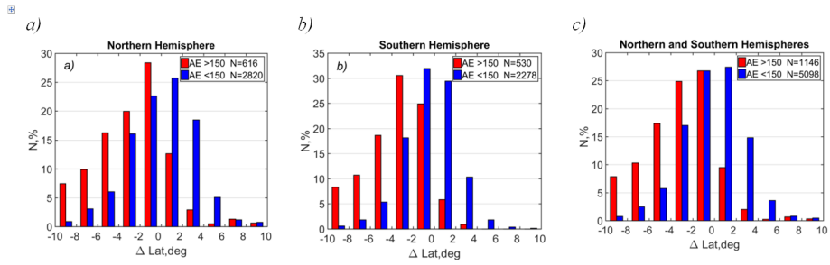
Figure 2.2: The distribution of \Delta \text{Lat} for AE > 150 nT (red bins) and < 150 nT (blue bins) for northern (a) and southern (b) and combined northern and southern (c) hemispheres
