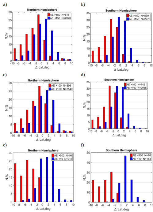
Figure 1.2: The distribution of \Delta Lat for AE >150 nT and <150 nT (a,b) for AE >100 nT and <100 nT (c,d) and for AE >500 nT and <10 nT (e,f) for northern (a,c,e) and southern (b,d,f) hemispheres
