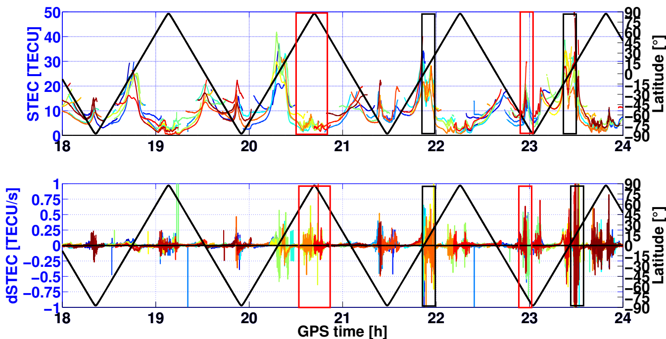
Figure 4. STEC (top) and its rate (bottom) for Swam A from 18:00 to 24:00 on DoY, 333, 2015. The right legend shows the geographic latitude.
