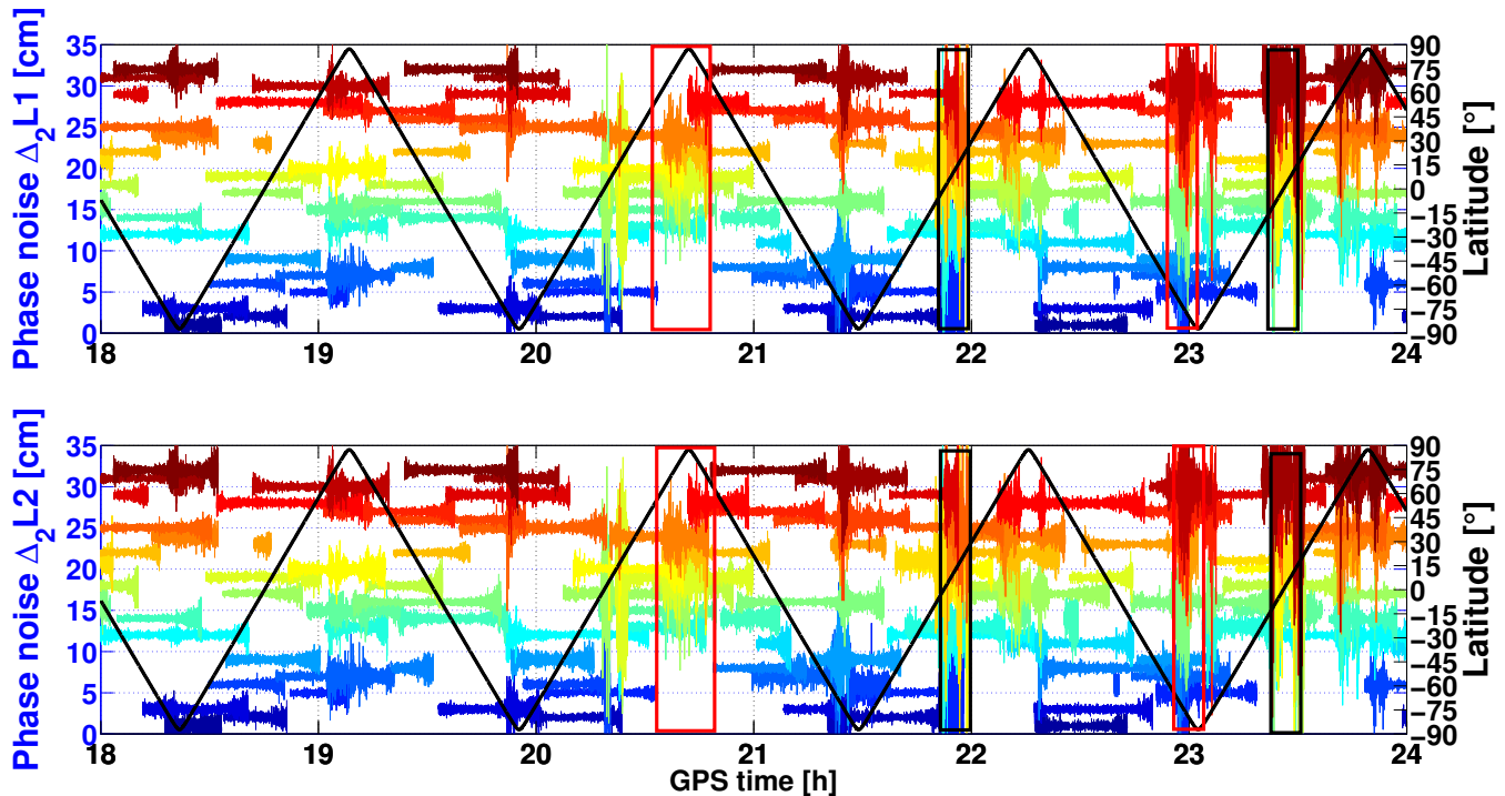
Figure 3. \Delta_2 L_1 (top) and \Delta_2 L_2 (bottom) noise for Swam A from 18:00 to 24:00 on DoY, 333, 2015, color coded per PRN (from blue PRN 1 to red PRN 32). The time series are intentionally shifted by \text{PRN} \times 1 cm. The local time is 8:30 for descending arc and 20:30 for ascending arc. The right legend shows the geographic latitude.
