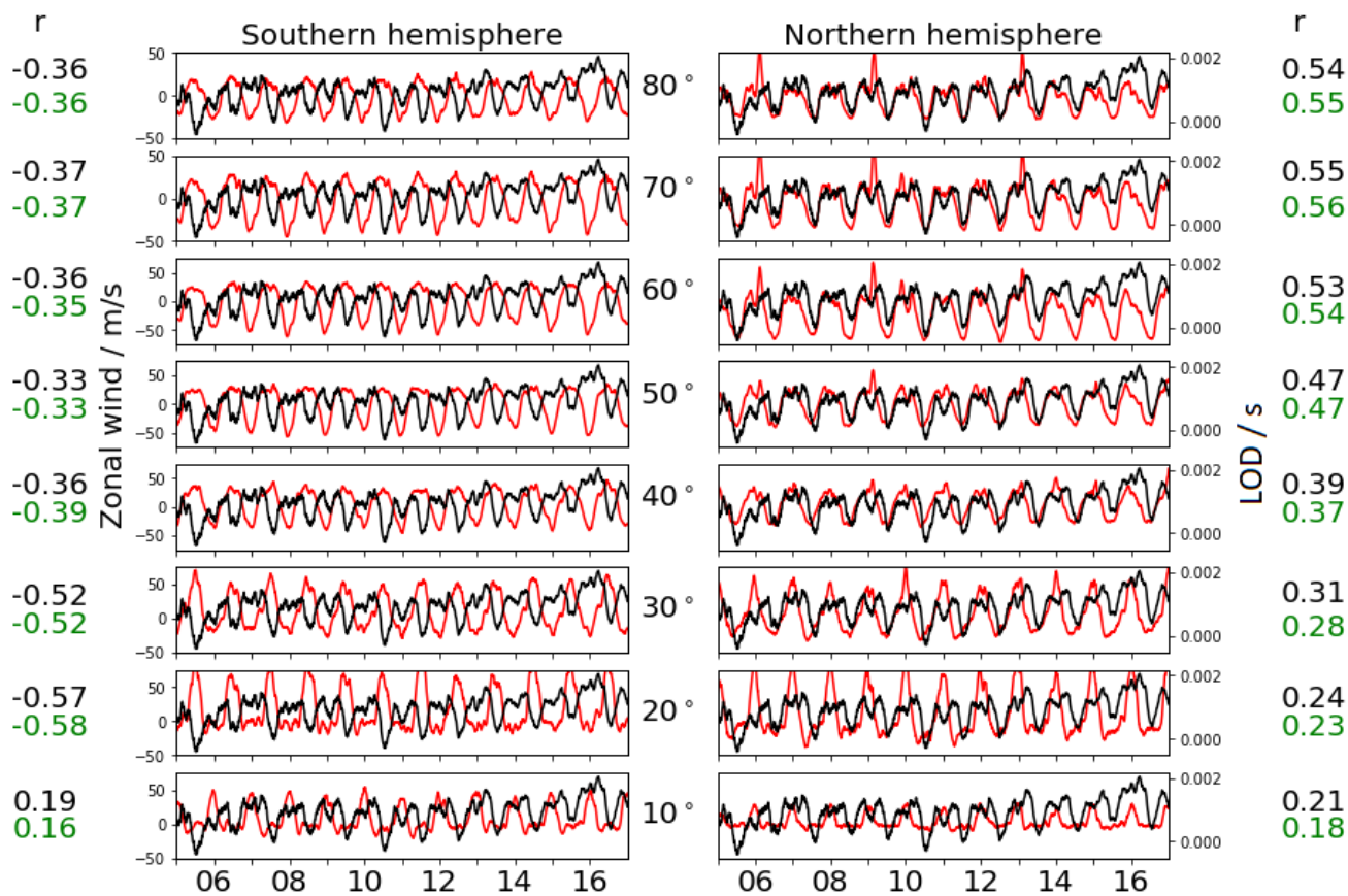
Figure 8. Zonal MLS wind (red) and LOD (black) at \sim 80 km geometric height for 0^\circ - 20^\circ E. The left part show the values for the southern hemisphere, the right for the northern hemisphere, for every 10^\circ latitude. The black correlation coefficients ( r ) are estimated for the mean between 0^\circ E and 20^\circ E, and the green coefficients corresponds to global average over all longitudes.
