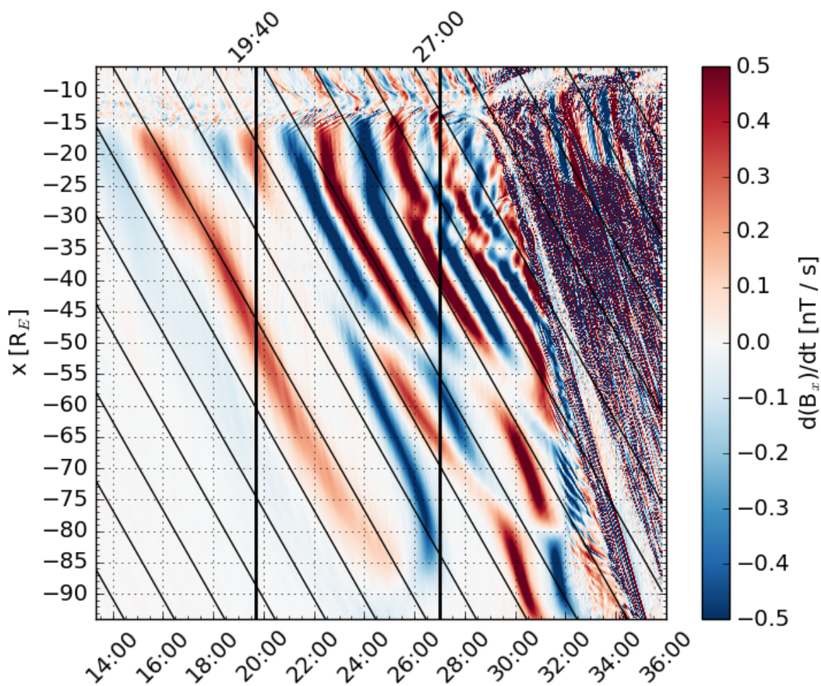
Figure 2. The same as Fig. 1 except that the color shows the time derivative of B_x . The color scale has been saturated to better show the relevant structures.
