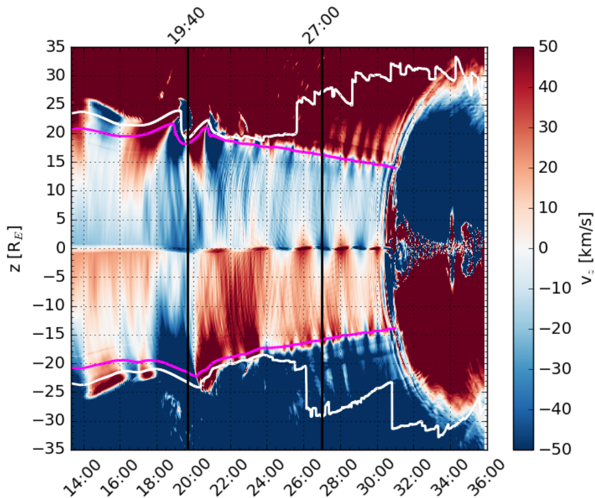
Figure 8. North component of the ion bulk velocity ( V_z ) as a function of z and time at y = 0 and x = -40 R_E . The vertical black lines are the same as in Fig. 1. The white and magenta (only plotted until 31:00) curves indicate the innermost boundaries where \beta_{\perp} > 1 and \beta_{\perp} > 0.1 in the region |z| > 5 R_E , respectively. The tail lobes are estimated to lie between the white curves and the magnetosonic wave resonance cavity between the magenta curves.
