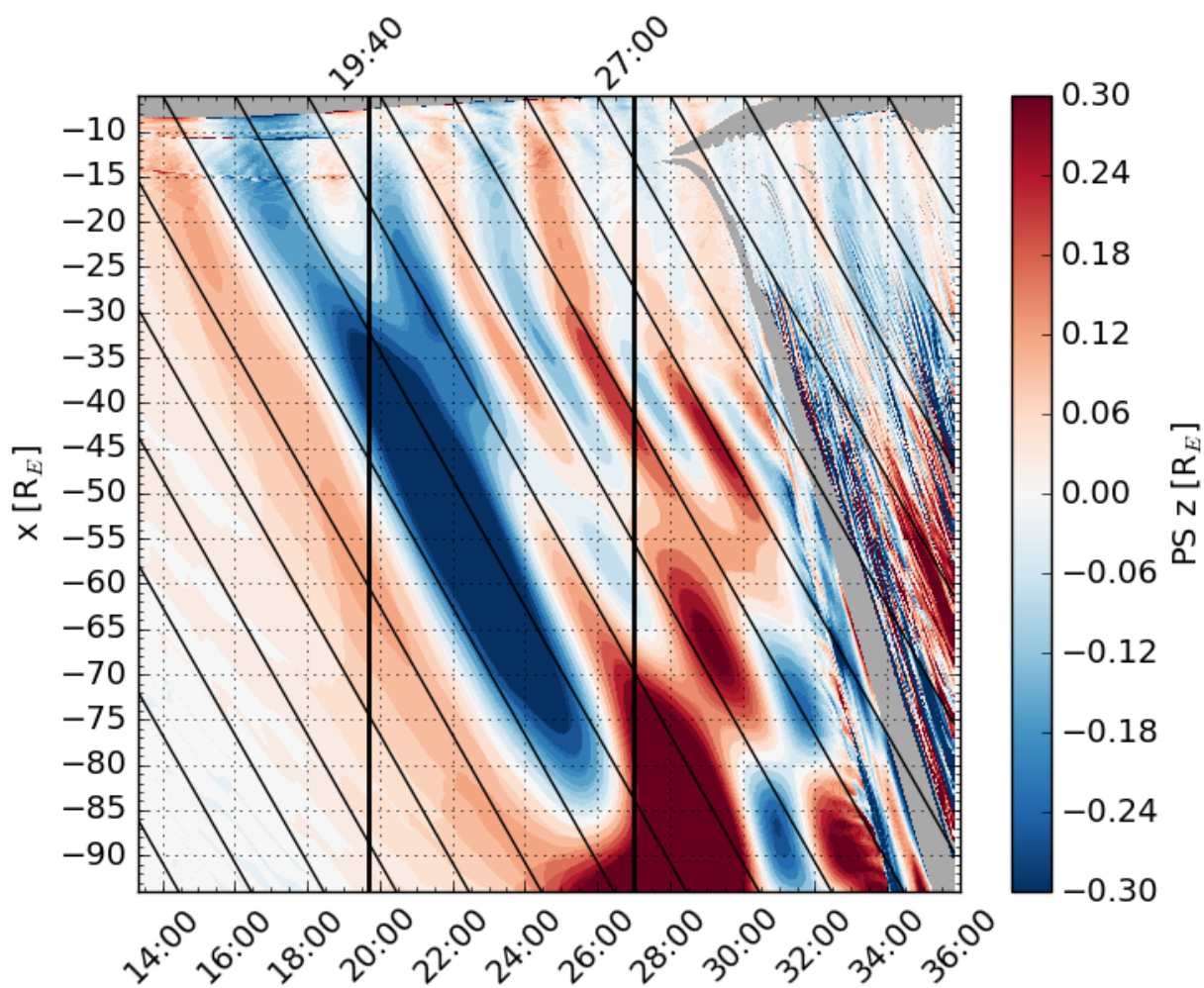
Figure 4. The same as Fig. 1 except that the color shows the location of the plasma sheet center in the z direction. Gray areas indicate regions where the location could not be determined.
