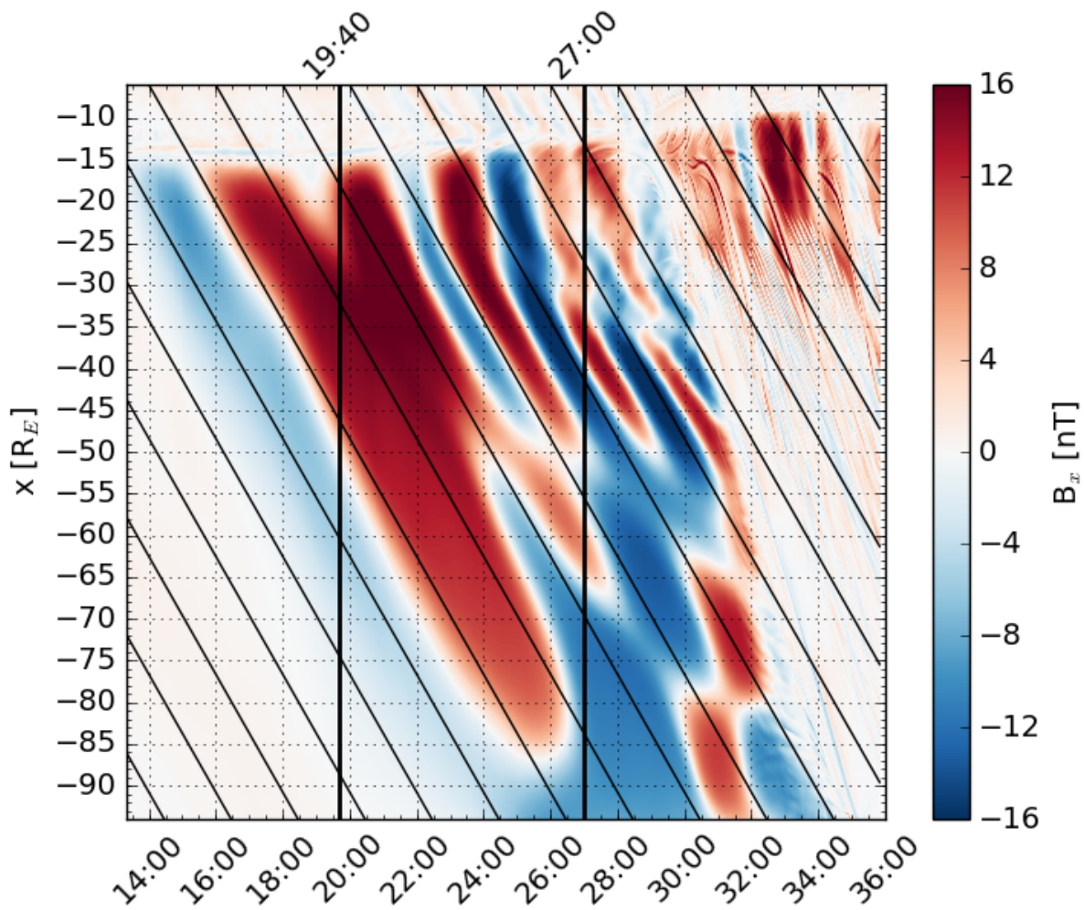
Figure 1. Earthward component of the magnetic field ( B_x , color) at the nominal position of the tail current sheet ( y = z = 0 ) as a function of x and time (MM:SS). The tilted black lines indicate motion at the solar wind velocity V_x = -750 km/s. The vertical black lines at 19:40 and 27:00 mark the time of Fig. 7 and the onset time of tail reconnection at x \approx -14 R_E , respectively.
