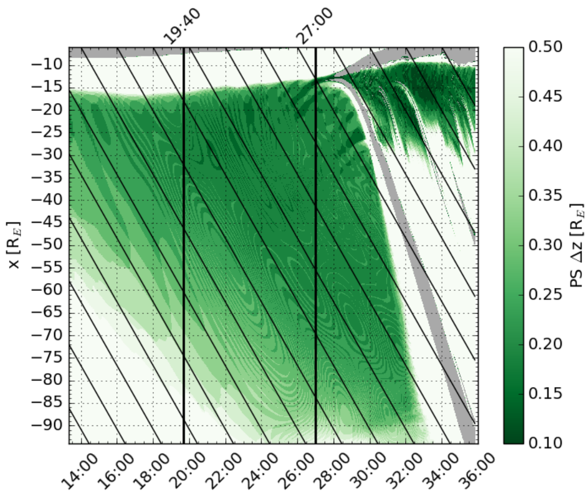
Figure 5. The same as Fig. 4 except that the color shows the plasma sheet thickness.
