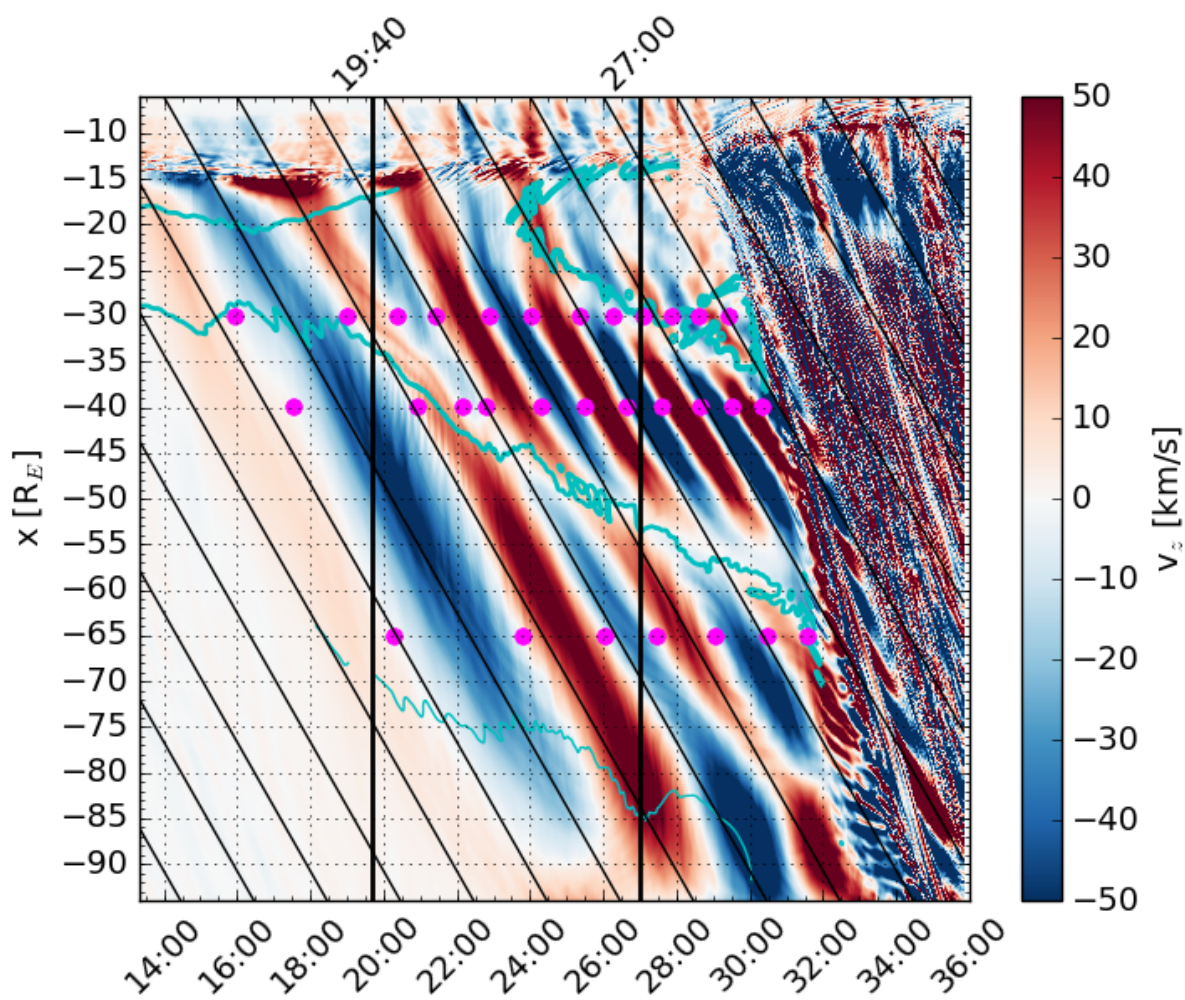
Figure 3. The same as Fig. 1 except that the color shows the north component of the ion bulk velocity ( V_z ). The cyan curves indicate isocontours of pressure in the z direction ( P_{magnetic,z} + P_{thermal,z} ) with a thicker curve indicating higher pressure: 0.05 nPa, 0.1 nPa, and 0.2 nPa. The magenta dots mark identified flapping half periods at x = -30 R_E , x = -40 R_E , and x = -65 R_E .
