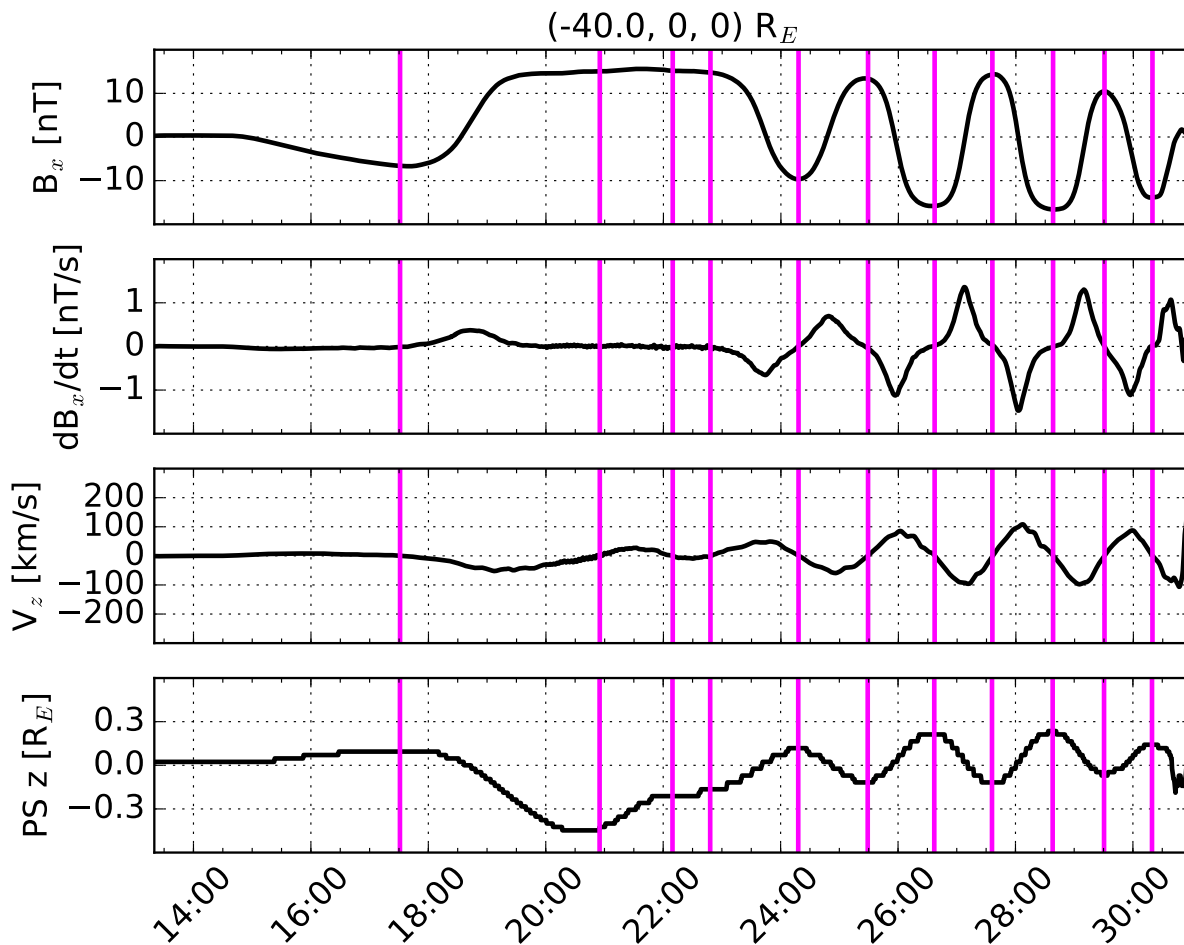
Figure 6. Time series observed by a virtual satellite located at x = -40 R_E and y = z = 0 in the simulation. From top to bottom, the parameters shown are: Earthward component of the magnetic field ( B_x , cf. Fig. 1), time derivative of B_x ( \partial B_x / \partial t , cf. Fig. 2), north component of the ion bulk flow ( V_z , cf. Fig. 3), and location of the plasma sheet center in the z direction (PS z , cf. Fig. 4). The vertical magenta lines identify flapping half periods based on sign changes of V_z , and they correspond to the magenta dots at x = -40 R_E in Fig. 3.
