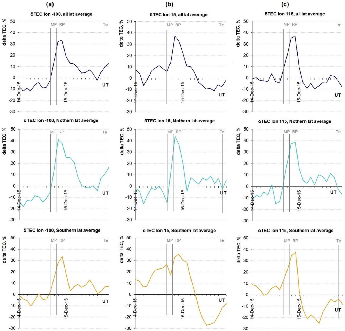
Figure 6: Results for storm #1: \delta TEC averaged along the whole meridian (upper panels), along the Northern hemisphere latitudes (middle panels) and along the Southern Hemisphere latitudes (lower panels) at the American (column a), Euro-African (column b) and Asian-Australian (column c) meridians. MP and RP beginnings and Te are marked by vertical lines.
