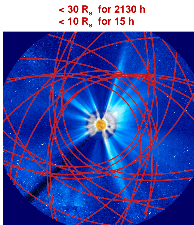
Parker Solar Probe , launch 2018 NASA, minimum perihelion 9.86 R_s
