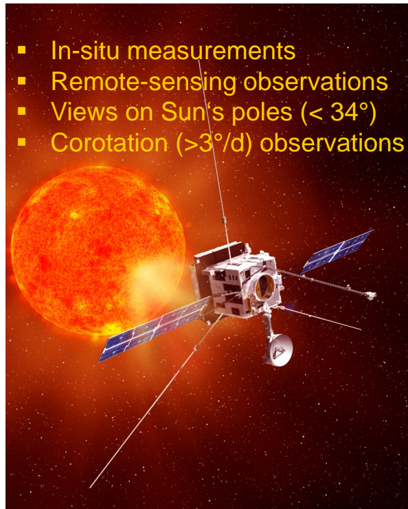
Solar Orbiter , launch 2020 ESA, minimum perihelion 59.6 R_s
