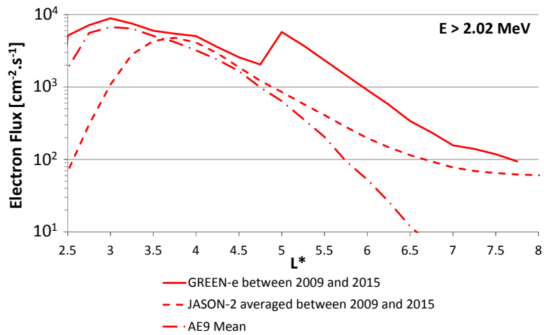
Figure 17: Mean electrons fluxes at JASON-2 orbit between 2009 and 2015 from GREEN-e (in full line), JASON-2 measurements (in dashed line) and from AE9 Mean v1.5 (dash-dotted line) for E > 2.02 MeV electrons.
