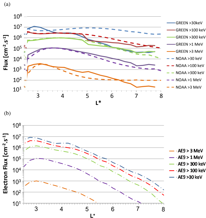
5 Figure 16: (a) Mean electrons fluxes at LEO orbit between 1999 and 2010 from NOAA-POES measurements (in dashed lines) and from one solar cycle in GREEN-e (in full lines) for several energy channels. (b) Electron fluxes at LEO orbit (820km,98°) from AE9 V1.5 Mean.
