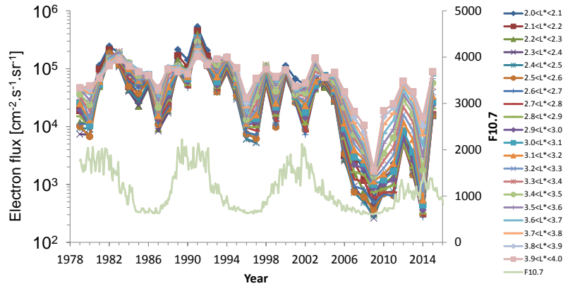
5 Figure 6: Electron >300 keV fluxes versus time (1978-2015) from all NOAA-POES data for each L^* intervals defined in the SLOT model. F10.7 is also represented in green
