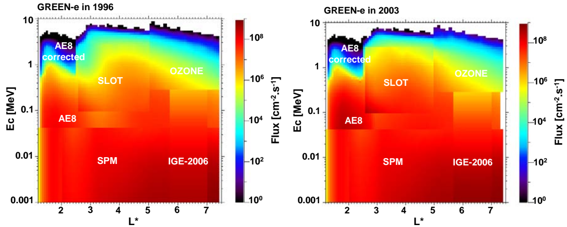
Figure 13: Electron fluxes versus L^* and energy in 1996 and 2003 provided by the GREEN-e model
