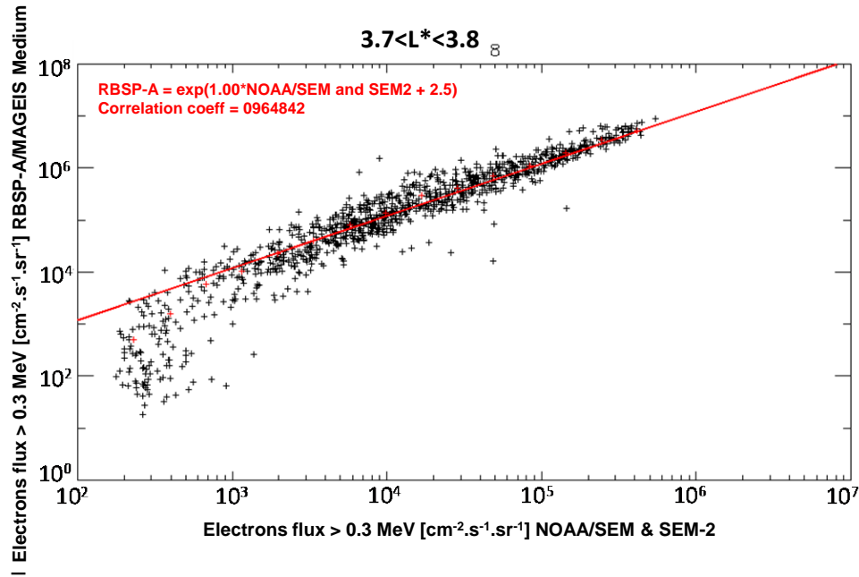
Figure 4: Example of correlation between NOAA-POES and Van Allen probe-A flux for electrons >0.3 MeV and for L* between 3.7 and 3.8
