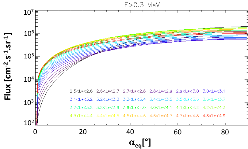
5 Figure 5: Electrons flux along magnetic field lines (90° corresponds to equator) for energy > 0.3 MeV and for all L* intervals of the SLOT model (in color)
