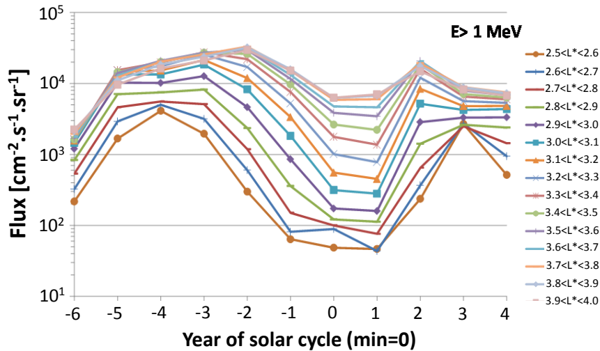
Figure 7: Electron >1 MeV fluxes versus year of solar cycle from all NOAA-POES data for each L^* intervals defined in the SLOT model
