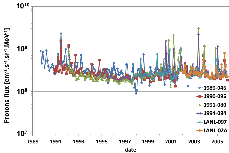
Figure 10: Monthly average 1keV proton flux measured at GEO by the detector MPA on board the different LANL satellites
