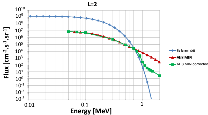
Figure 3: Electron fluxes provided by Salammbô in blue (averaged on years during solar minimum), by AE8 MIN in red and AE8 MIN corrected in green at L=2
