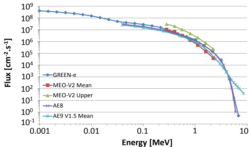
5 Figure 15: Electron spectrum from GREEN-e (in blue) on a whole solar cycle compared to the mean (in red) and upper (in green) flux provided by MEO-V2 model
