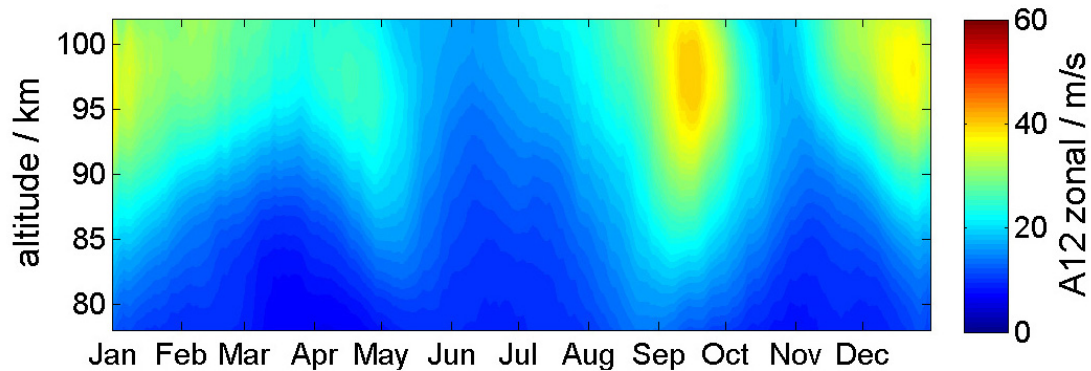
Fig. 1. Amplitudes of semidiurnal tides extracted from the Canadian meteor data (43 deg N) using the same adaptive filtering technique.
