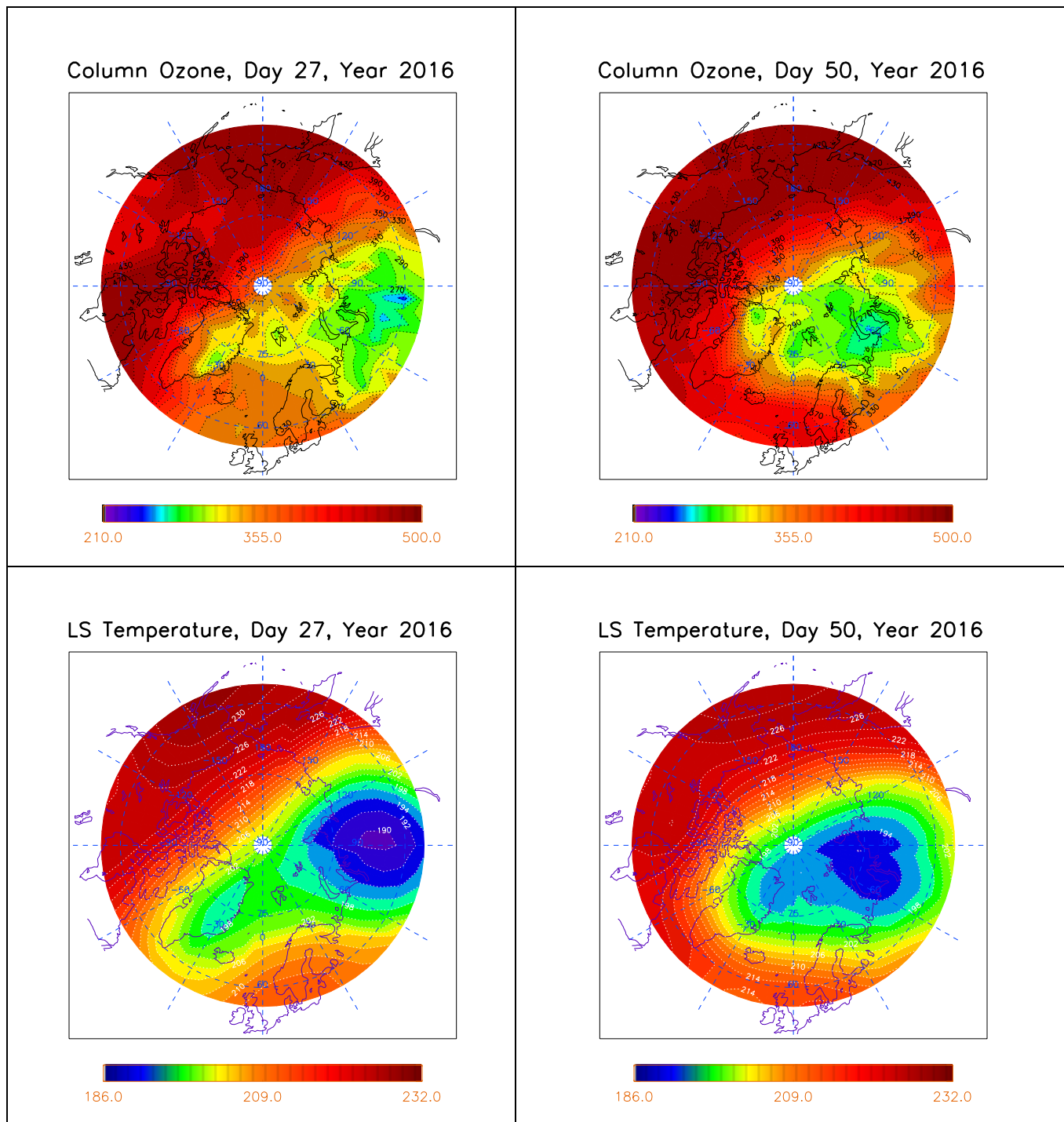
Figure 4: Column ozone (DU) for the days with minimum local registered values (January, 27 ( left ) and February, 19 ( right )), simulated with the RSHU model ( top ) and temperature of the lower stratosphere (K) from MERRA reanalysis ( bottom ).
