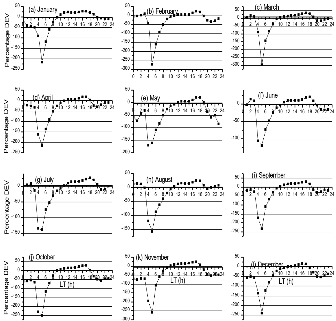
Figure 6: Percentage deviation of IRI-2016 from OBS-TEC for year 2012
