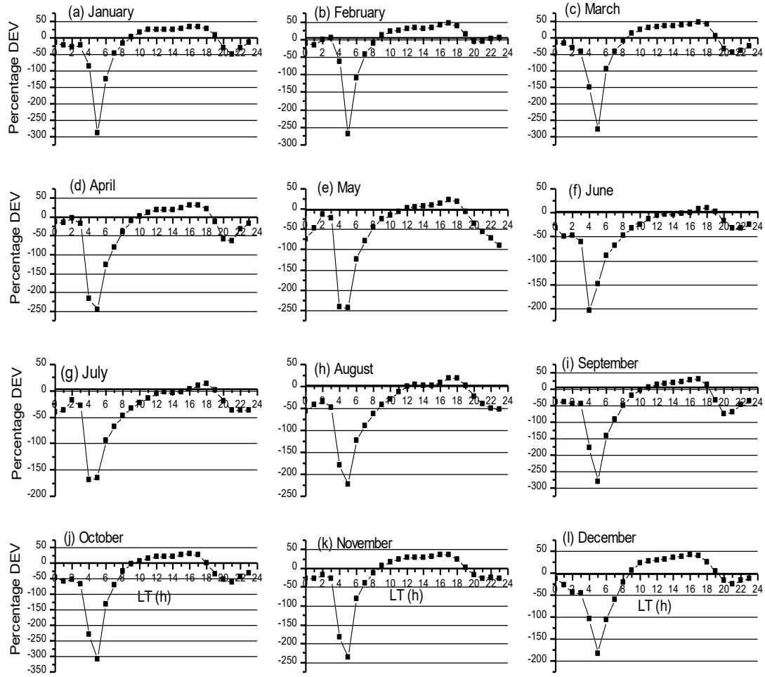
Figure 8: Percentage deviation of IRI-2016 from OBS-TEC for year 2014
