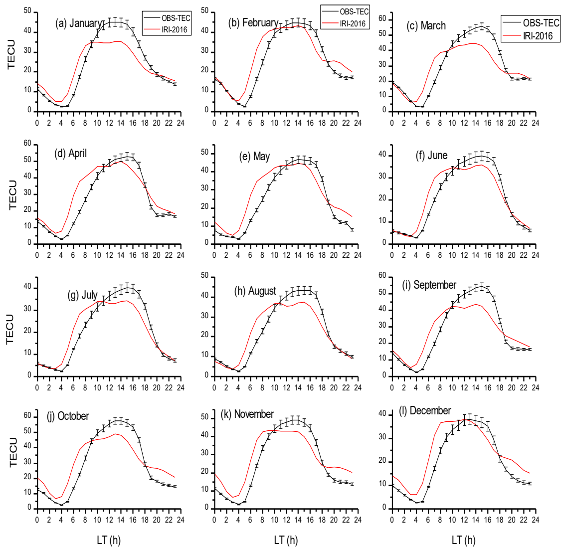
Figure 2: Same as Figure 1 for 2012.
