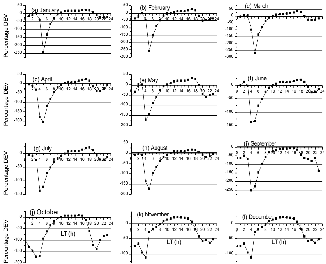
Figure 7: Percentage deviation of IRI-2016 from OBS-TEC for year 2013
