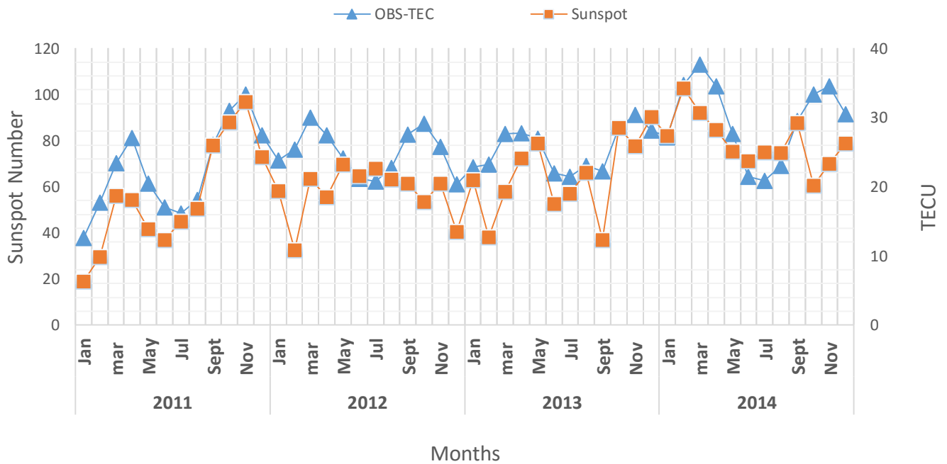
Figure 10: Annual variation of OBS-TEC and sunspot number, Rz
