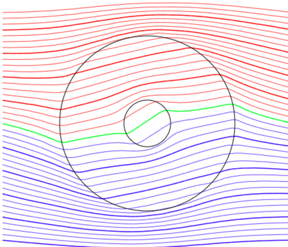
Fig. 1. Equipotential contours that satisfy [\text{div}(\mathbf{C})] for two concentric patches of density 2x and 5x the background density, and a uniform [\kappa]=1 . Although the E field and the boundary
