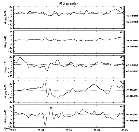
Figure 3' The Pi 2 observed by FSM, FSMI, WHI, LARG and ATHA between 09:25 and 09:55 UT.
