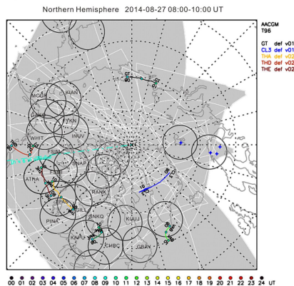
Figure 1 The spacecraft footprints and Ground-Based Observatory.
