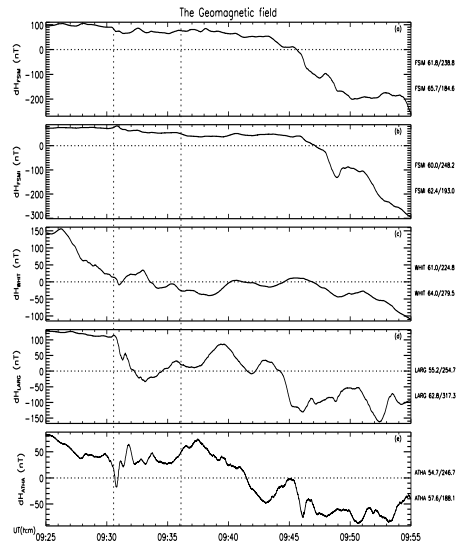
Figure 2 Geomagnetic field observed by FSIM, FSML, WHIT, LARG and ATHA between 09:25 UT and 09:55 UT.
