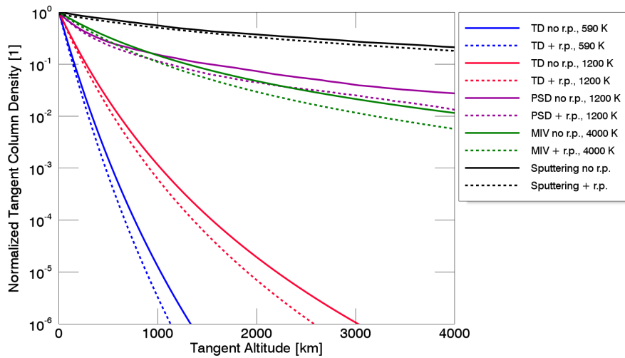
Figure 2. Column density profiles as a function of tangent altitude for Na where the column density at the surface is normalized to one, and for the different release mechanisms: TD, PSD, MIV, and SP with and without radiation pressure (r.p.) centered at subsolar point and for different surface temperature values. The simulation was done with an ensemble of 10^6 particles, and Mercury at a TAA= 158^\circ and R_{orb} = 0.458 AU.
