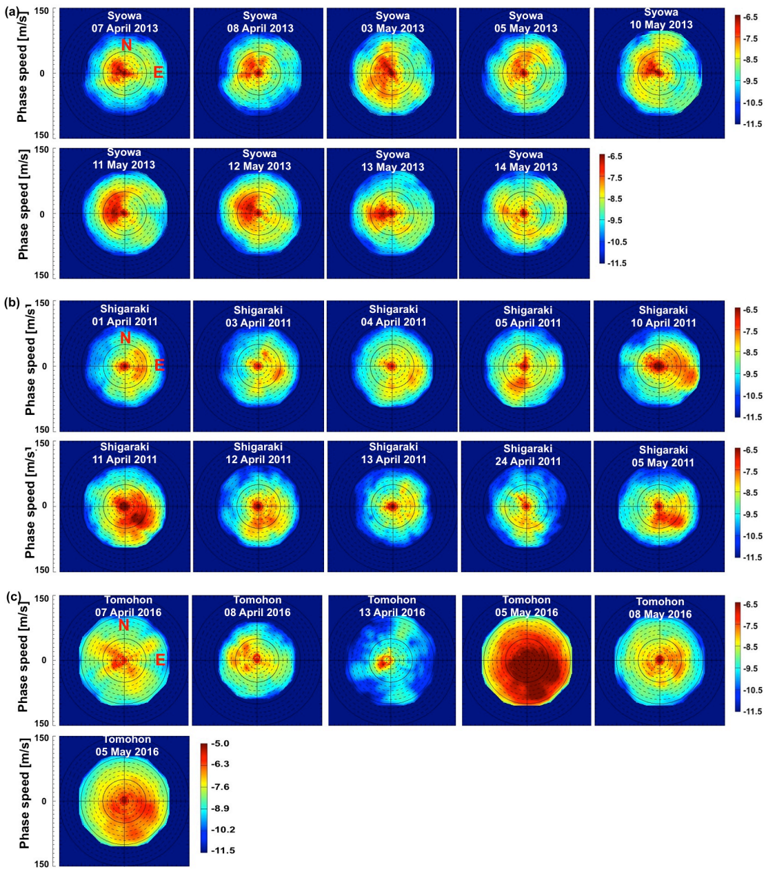
Figure 3: Day-to-day variation of 2D phase velocity spectra for April–May 2013 at the Syowa Station (a), in Shigaraki (2011) (b), 5 and in Tomohon (2016) (c). Figure 3c is the same as that for May 5, 2016, but with a different color bar level to better visualize the dominant wave propagation direction.
