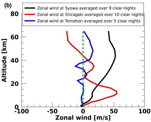
Figure 4: (a) Average day-to-day variation of the 2D phase velocity spectrum of AGWs observed at Syowa, in Shiragaki, and in Tomohon. (b) Average zonal wind profiles (positive: eastward) and (c) average meridional wind profiles (positive: northward) of GWs observed during clear nights from MERRA-2 data.
