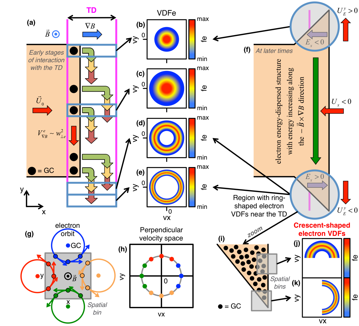
Figure 4: Panel (a) illustrates the phase A of plasma jet's interaction with the magnetic discontinuity. The black dots indicate the guiding centres (GCs) of electrons localized in the front edge. The multiple groups of green-yellow-red arrows show the gradient-B drift displacement of the GCs proportional to the gyration energy (green corresponds to the lowest energy). The four blue boxes indicate the bins where the VDF is computed. The electron VDFs obtained for the upper edge bins (panels (b) and (c)) are gyrotropic and their phase density vanishes for large velocities; the VDFs obtained for the bottom edge bins (panels (d) and (e)) are ring-shaped. Panels (g) and (h) illustrate how the electrons with GCs outside a spatial bin contribute to different sectors of the VDF collected in the respective bin. The colours of the dots in panel (h) identify which particle shown in panel (g) contributes to that sector of the VDF. This effect corresponds to a remote sensing of the large Larmor radius electrons outside the bin. Panels (f), (i)–(k) show how the remote sensing effect contributes to the formation of crescent-shaped VDFs in a configuration similar to the PIC simulations.
