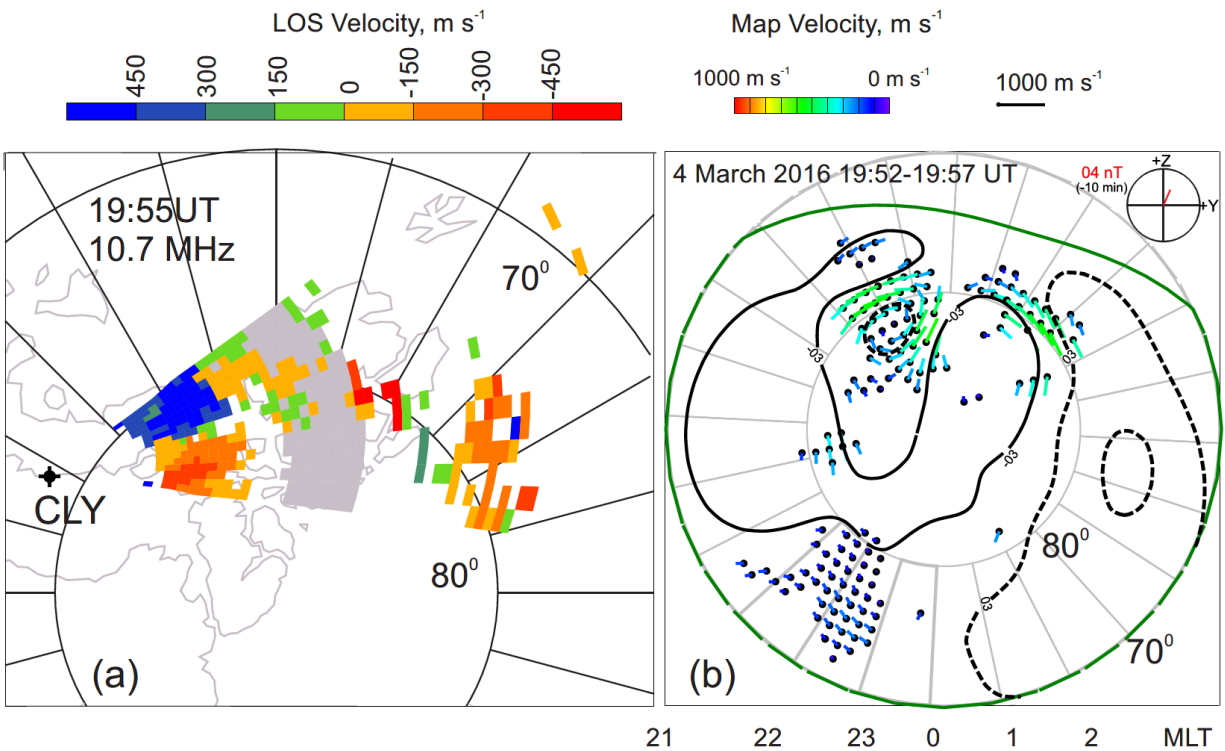
365 Figure 6: (a) A CLY LOS velocity map at 19:55 UT on 04 March 2016 and (b) a 5 min convection map calculated from all SuperDARN radar measurements for the same period of time. The TS2018 statistical model (Thomas and Shepherd, 2018) of the order 8 for the solar wind electric field of 2.1 mV/m was used. Contours of the electric potential are 6 kV apart.
