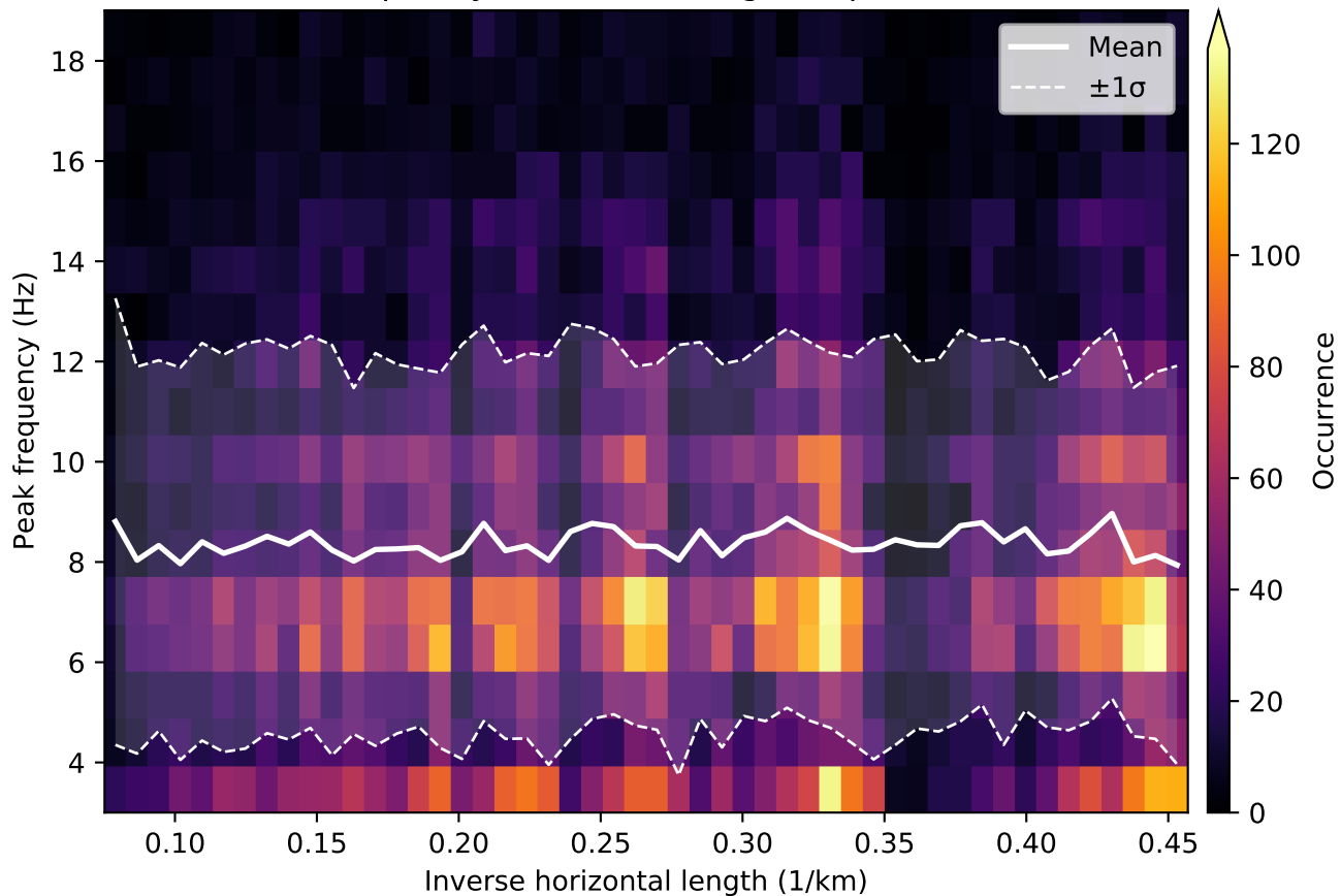
Frequency vs. inverse length of patches
