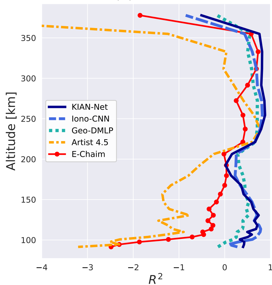
(a) R^2 -score
