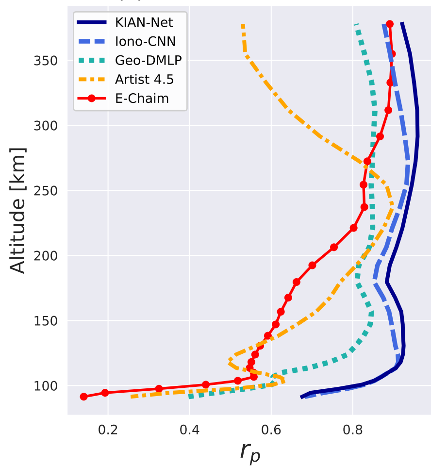
(c) Pearson's Correlation
