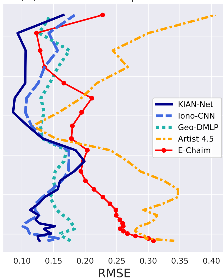
(b) Root Mean Squared Error
