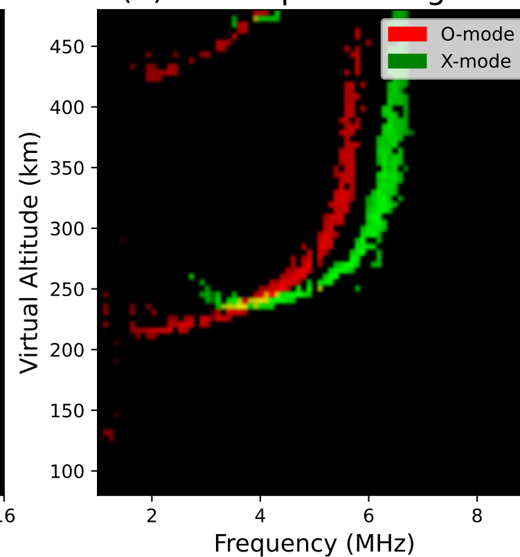
(b) Resampled Ionogram
