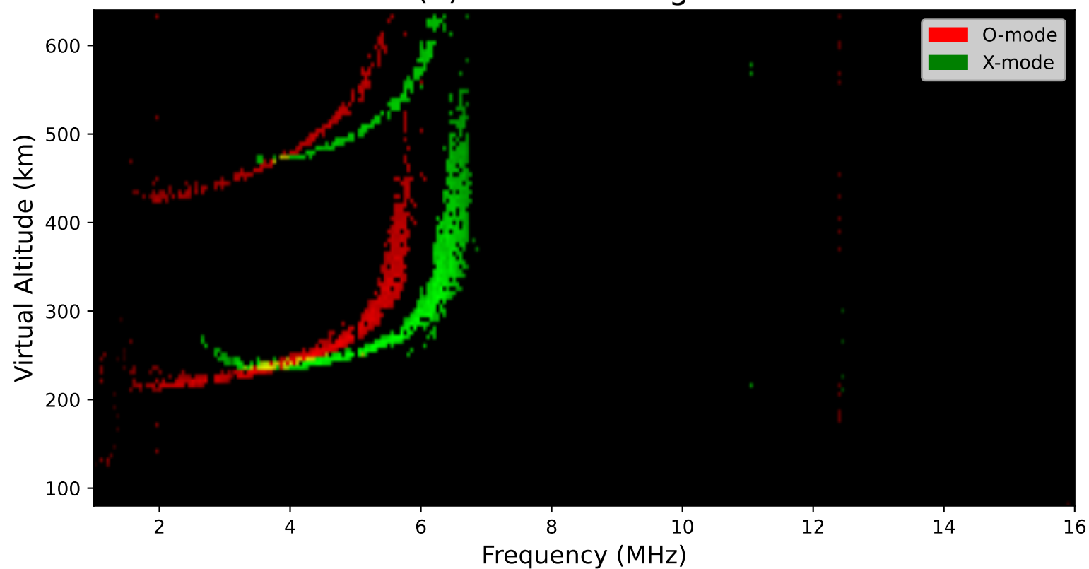
(a) Filtered Ionogram
