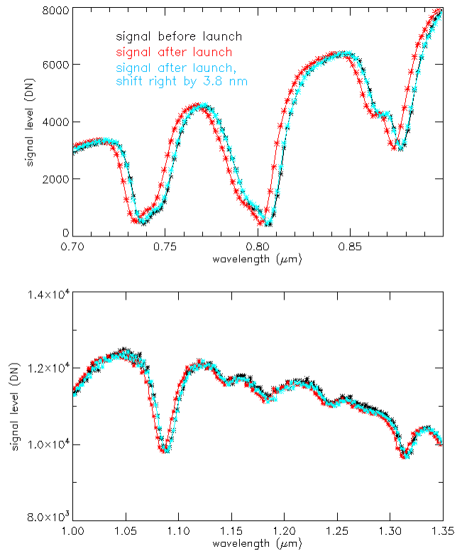
Figure 7. Straylight corrected signal near the left edge of the FOV from the ICU lamp before and after launch; top panel: Spectral range with strong didymium absorptions; Bottom panel: Spectral range with no strong spectral features from the QTH lamp; A scaling factor has been applied to the signal after launch (1.08 for the top panel, 1.12 for the bottom panel) so as to compensate for the decrease in the ICU lamp signal from before to after launch near the left edge of the FOV (see Sect. 3.2.1).
