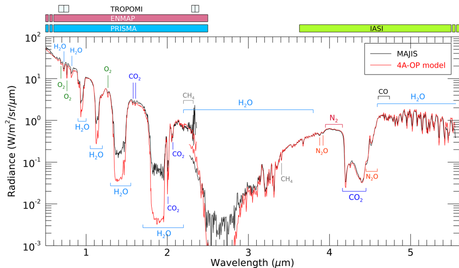
Figure 1. MAJIS VISNIR spectrum extracted from cube C17 (#20240820214813, pixel [42,400]) and MAJIS IR spectrum extracted from cube C15 (#20240820214628, pixel [20,10]) compared to radiative transfer simulations from the 4A/OP model specific to the observational and atmospheric conditions of the VISNIR and IR spectra (see text for details). Main atmospheric gaseous absorptions and the spectral ranges/operating bands of the PRISMA, TROPOMI, ENMAP and IASI instruments used for comparison with MAJIS in this section and in Sect. 4 are also indicated. The main focus is on the wavelength of spectral absorption features as their strength depend on spatially variable column densities.
