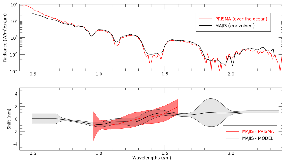
Figure 3. Top panel: Best collocated and concomitant PRISMA spectrum (red) and MAJIS VISNIR spectrum (black). The observations are both over the Earth's ocean; bottom panel: Spectral residuals between the MAJIS and PRISMA spectra presented in the top panel are shown in red with their 1\sigma -uncertainties envelop. The spectral residuals with respect to the 4A/OP radiative transfer model for the same MAJIS pixel (from Fig. 2a) are shown in black with their 1\sigma -uncertainties envelop for comparison.
