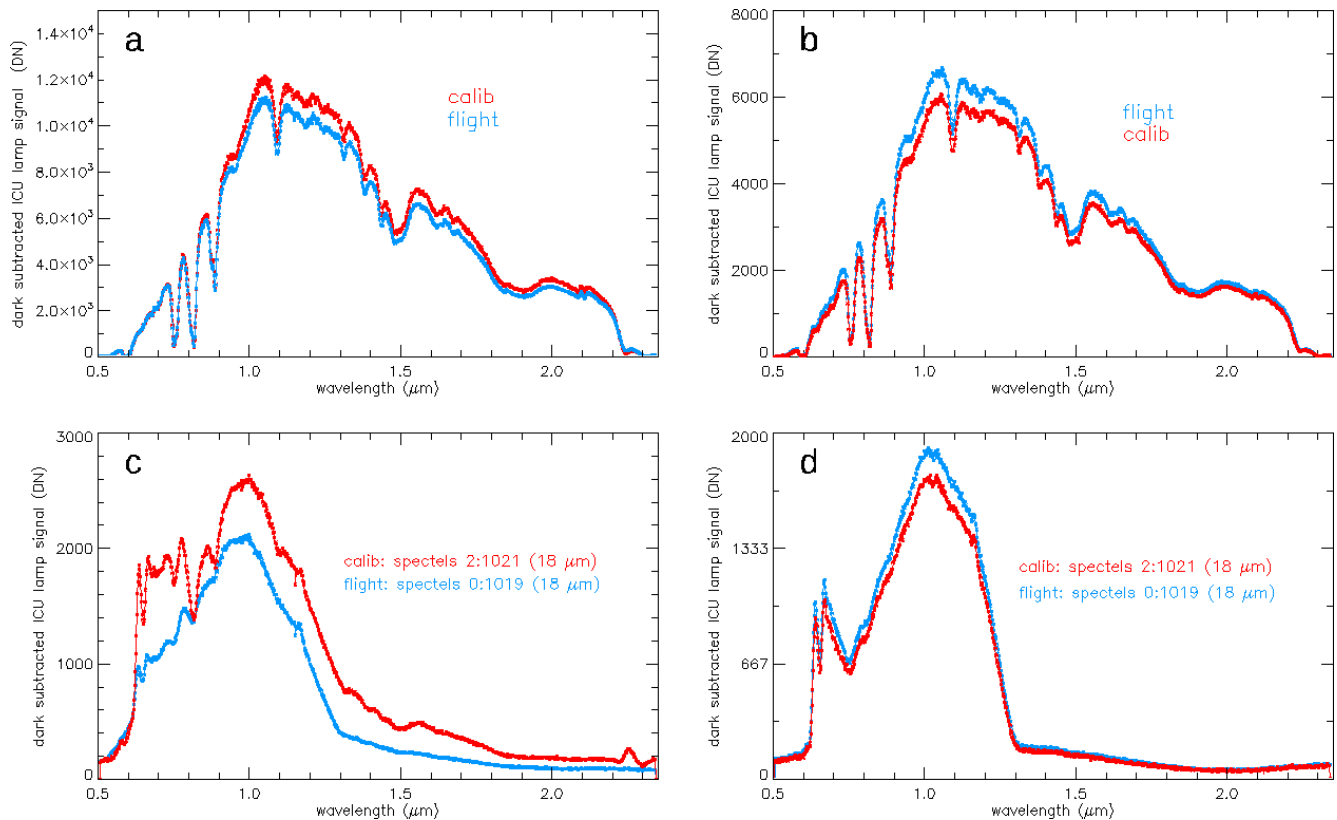
Figure 13. Legitimate signal and straylight contribution for observations of the ICU lamp with the VISNIR channel during ground calibration (“calib”) and after launch (“flight”). The legitimate signal for a region near the left edge of the FOV is presented in panel (a) and that for a region near the right edge of the FOV in panel (b). The straylight contribution beyond the left edge of the FOV is presented in panel (c) and that beyond the right edge of the FOV in panel (d). The ICU spectra during flight have been shifted by 2 HIRG spectels so as to compensate for the spectral shift reported by Haffoud et al (2024), and updated in Sect. 2.
