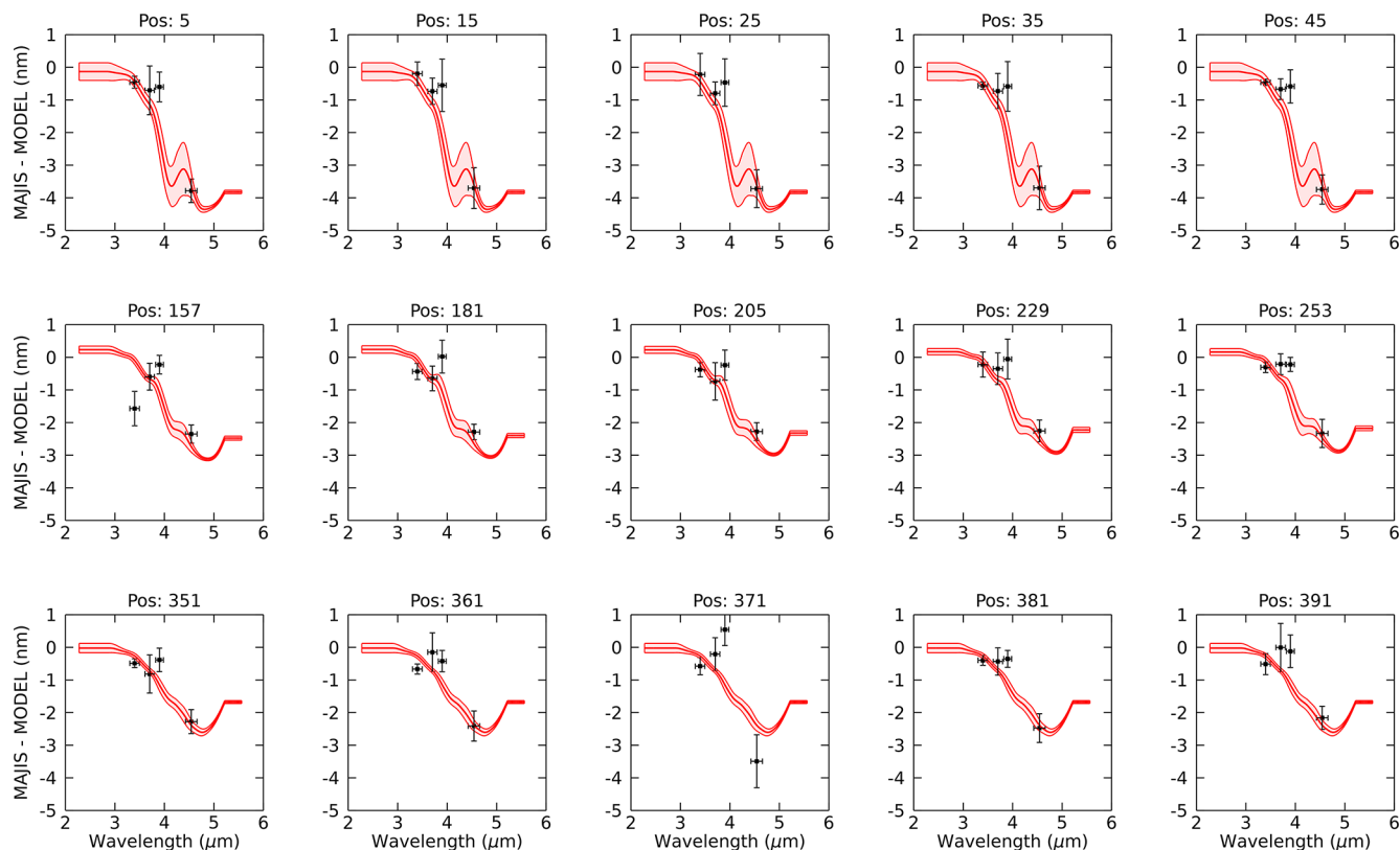
Figure A1. The spectral residuals from the joint retrievals of the spectral residuals and FWHM in the 4 spectral ranges detailed in the main text are presented as black squares, along with their 1\sigma -uncertainties, for the 26 positions along the MAJIS slit indicated in nominal pixels on top of each panel (see also Table 1). Error bars along the wavelengths dimension indicate the width of the spectral interval over which the retrievals have been performed. These retrievals are compared with the estimation of the spectral residuals using the entire MAJIS IR channel presented in Sect. 2.1.1 and in Fig. 4 (red curve with 1\sigma -uncertainty envelop).
