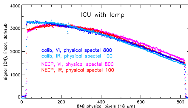
Figure 6. Spatial profile of the ICU signal before and after launch. The profiles obtained during calibration and 2 months after launch (Near Earth Commissioning Campaign, NECP) are shown for a VISNIR HIRG spectel (spectel 800, 1.952 \mu\text{m} ) and for an IR HIRG spectel (spectel 100, 2.58 \mu\text{m} ). These two spectels have been selected as they provided very similar raw signal levels across the field of view (FOV).
