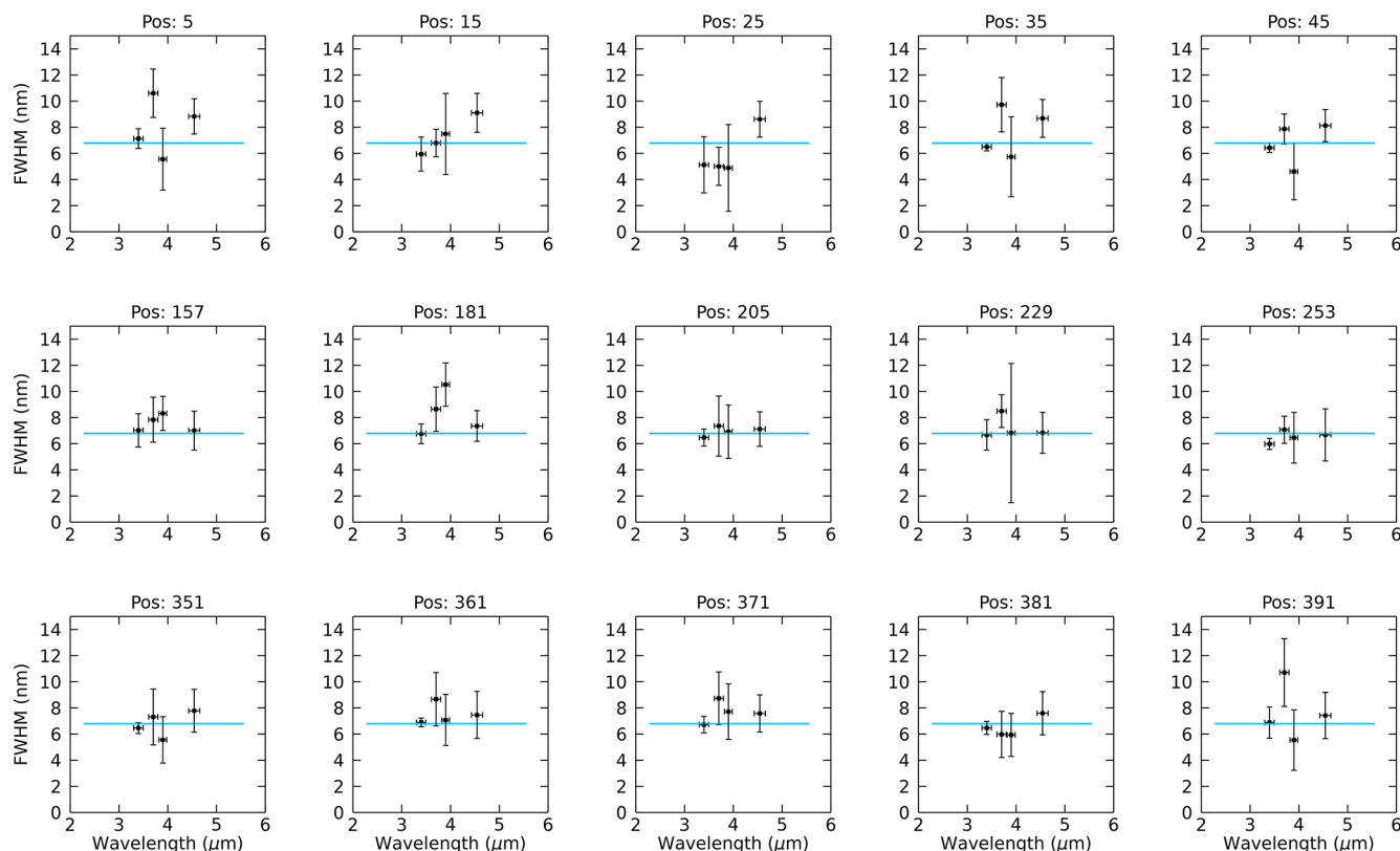
Figure A2. Same as Fig. A1 but for the FWHM estimation from the joint retrievals of the spectral residual and FWHM. The blue line shows the reference FWHM in the IR channel (a constant 6.8 nm value in the case of nominal pixels) as recommended by Haffoud et al. (2024) from on-ground calibration measurements.
