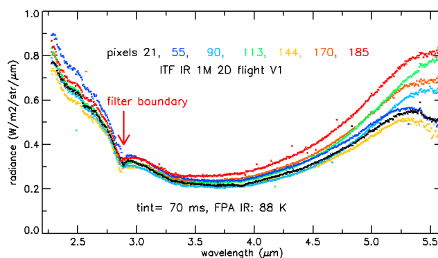
Figure 10. Radiance spectra of the Moon obtained over the left half of the FOV after the first stage of ITF adjustment. The 7 spectra correspond to MAJIS pixels ( 36\mu\text{m} pitch) from pixel 21 (close to the left edge) to pixel 185 (close to the center of the 400 pixels FOV).
