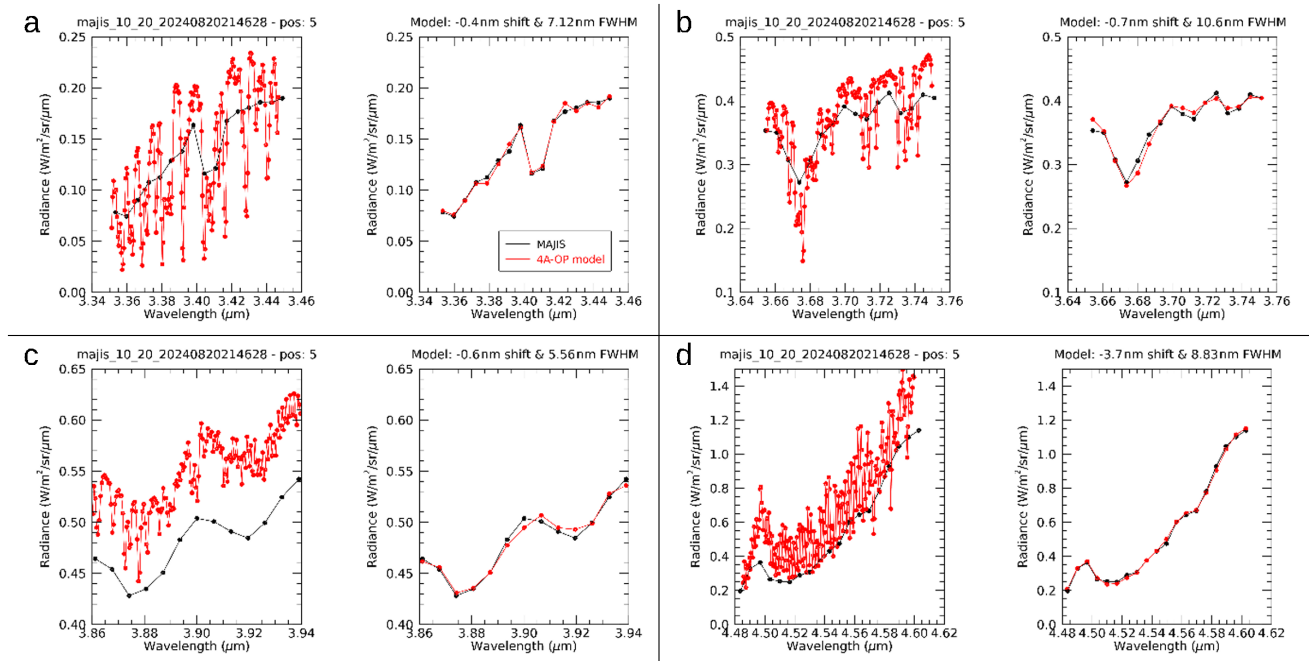
Figure 5. Examples of simultaneous retrievals of the spectral residual and the spectral width (FWHM) in 4 spectral ranges within the MAJIS IR channel, for the position 5 (in nominal pixels) of the MAJIS slit. Each spectral range includes a specific absorption band used for constraining both the CWL and FWHM at the nominal pixel level within the wavelength range of the IR channel; Panel (a): residuals and FWHM retrievals for the interval 3.35–3.45 \mu\text{m} including the \text{CH}_4 band at 3.4 \mu\text{m} . The black lines and dots display a MAJIS spectrum extracted from the cube C15 (#20240820214628) at the across-slit \times along-slit position [10, 5] in nominal pixels. Red lines and dots present the results of the 4A/OP model adapted to match the conditions of observation of the MAJIS spectrum, at 1 nm FWHM on the left of panel (a), and, on the right of panel (a), convolved with the FWHM and residuals needed to best fit the MAJIS spectrum (best fitting values of the residuals and FWHM are indicated above the graph on the left); Panel (b): Same as panel (a), but for the 3.65–3.75 \mu\text{m} interval including the \text{H}_2\text{O} band at 3.67 \mu\text{m} . Panel (c): Same as panel (a), but for the 3.86–3.94 \mu\text{m} interval including the double \text{N}_2\text{O} band at 3.875 and 3.92 \mu\text{m} ; Panel (d): Same as panel (a), but for the 4.48–4.6 \mu\text{m} interval including the \text{N}_2\text{O} band at 4.51 \mu\text{m} .
