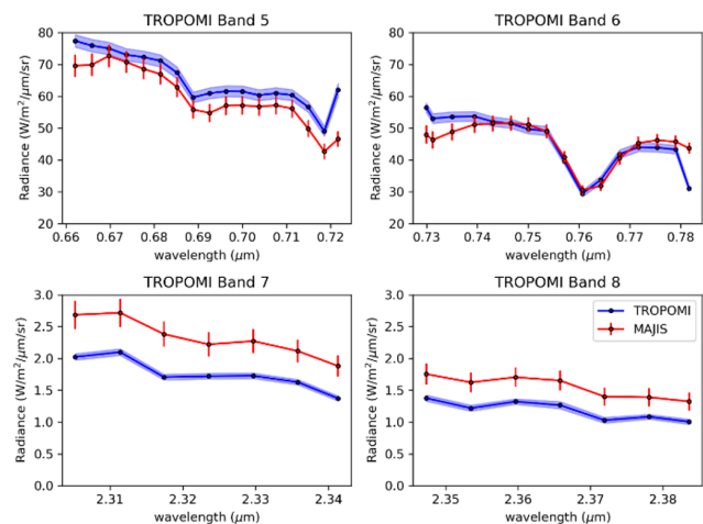
Figure 20. Averaged results of colocated TROPOMI and MAJIS radiances for MAJIS observations C15 and C17. The blue shaded area represents the TROPOMI total uncertainty, and the red error bars represent the MAJIS total uncertainty, the largest contribution resulting from the variability within sets of co-located MAJIS pixels corresponding to a single TROPOMI pixel.
