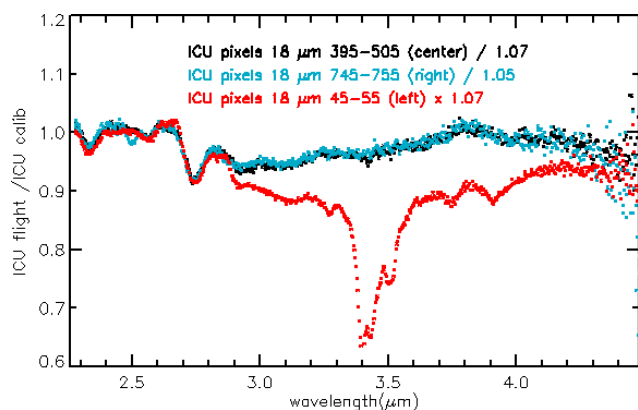
Figure 9. ICU lamp signal after launch divided by the signal before launch near the center, the right edge and the left edge of the FOV. The ratios have been normalized by a factor smaller than 1 at the center and right of the FOV, larger than 1 left of the FOV so as to compensate for the evolution of the spatial profile from before to after launch (see Fig. 6).
