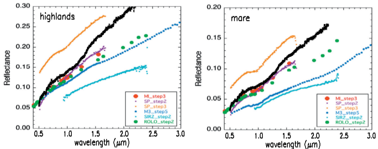
Figure 15. Lunar reflectance spectra from MAJIS observations (black stars) in the VISNIR spectral range (0.5–2.250 μm) corrected for straylight and assuming Lambert scattering for highlands (left panel) and for mare (right panel) compared to lunar reflectance spectra of highlands and mare obtained by other instruments (Ohtake et al., 2013).
