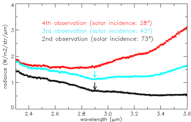
Figure 12. MAJIS radiance spectra obtained during three of the five observations of the Moon by MAJIS (see Poulet et al., 2026) applying the updated IR 2D-ITF. Blue and black arrows correspond to a possible weak OH signature at 2.9 \mu\text{m} for mid to high incidence MAJIS observations.
