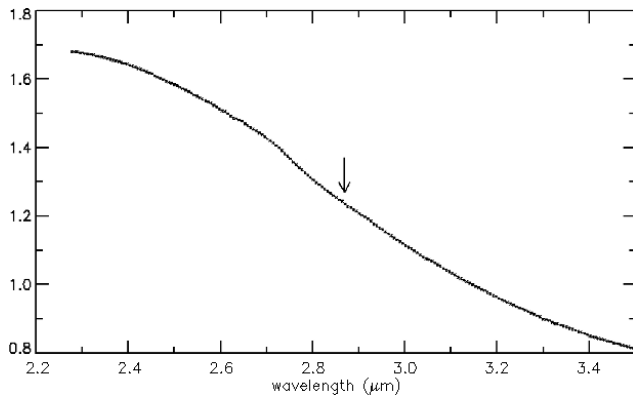
Figure 11. Ratio of radiances observed in the same MAJIS cube for highlands and mare areas. The arrow corresponds to the filter boundary at 2.880 \mu\text{m} .
