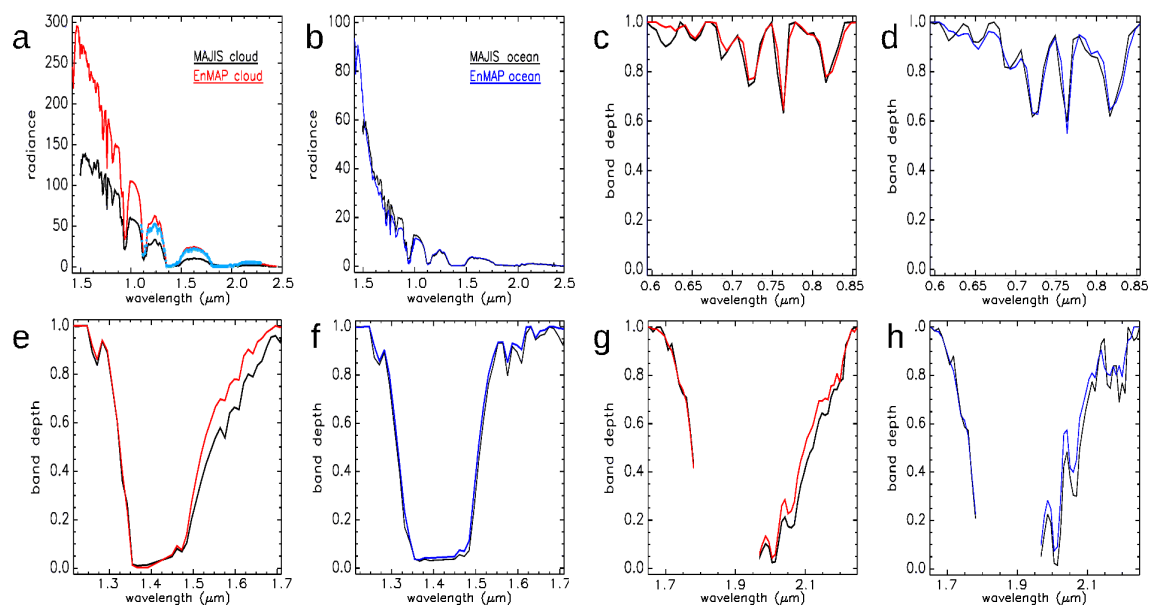
Figure 18. Panel (a): Radiance measured for the resampled ENMAP pixels and the MAJIS pixels selected as representative of cloudy areas; panel (b): Same as panel (a) for cloud-free areas. The light blue radiance spectrum in panel (a) is that of a MAJIS pixel farther North, with a continuous cloud cover, for wavelengths larger than 1.1 \mu\text{m} (at shorter wavelengths, it reaches saturation); panel (c): Continuum removed spectra from ENMAP and MAJIS in the 0.750 \mu\text{m} spectral range for cloudy areas; panel (d): Same as panel (c) for cloud-free areas; panels (e), (f): Same as panels (c), (d) for the 1.5 \mu\text{m} \text{H}_2\text{O} absorption band; panels (g), (h): Same as panels (c), (d) for the 2 \mu\text{m} \text{H}_2\text{O} absorption band (only wavelengths sampled by ENMAP have been displayed).
