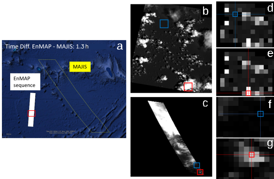
Figure 17. Panel (a): location of the ENMAP observation (white area) and the MAJIS observation (C17, yellow outline) over the Pacific Ocean; Panel (b): ENMAP radiance map at 0.75\ \mu\text{m} for the red rectangle in panel A, with the locations of the areas selected as representative of cloudy (red) and cloud-free (blue) ENMAP data; Panel (c): Radiance map at 0.750\ \mu\text{m} for the full MAJIS swath, with areas selected for cloudy (red) and cloud-free (blue) representative spectra. Panels (d), (e): Panel (b) resampled at the MAJIS resolution with the resampled pixels selected as representative of cloudy (red) and cloud-free (blue) areas; Panels (f), (g): Zoom on the red and blue areas in panel (c), indicating the MAJIS pixels selected as representative of cloud-free (blue) and cloudy (red) areas.
