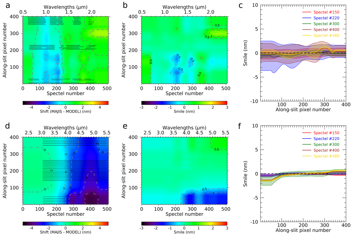
Figure 2. Panel (a): Map of the spectral residual (in nm) between MAJIS and reference 4A/OP simulated spectra for the VISNIR channel, as a function of the nominal spectel number (the corresponding wavelengths are indicated on the upper axis) and slit positions in units of nominal pixels; Panel (b): Same as (a) but for the VISNIR smile effect (in nm), i.e. the spectral residual at a given location and wavelength when compared to the central slit position, #200); Panel (c): Selection of transects through the smile map in (b) for spectels #150, 220, 300, 400 and 480, with their respective 1 \sigma -uncertainty envelope. Panels (d), (e) and (f): Same as panels (a), (b) and (c) for the MAJIS IR channel. In panels (a) and (d), black lines designate the actual spectral and spatial pixels used for the residual retrievals after removal of the outliers (see text for details). The maps showed in panels (a), (b), (d) and (e) have been obtained by bilinear 2D interpolation and smoothed by an averaging [50 spectels × 50 pixels] 2D boxcar.
