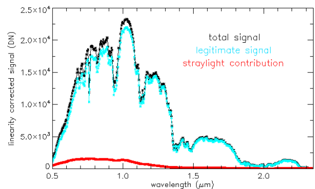
Figure 14. Total signal, legitimate signal and straylight contribution for an Earth spectrum from observation C17.
