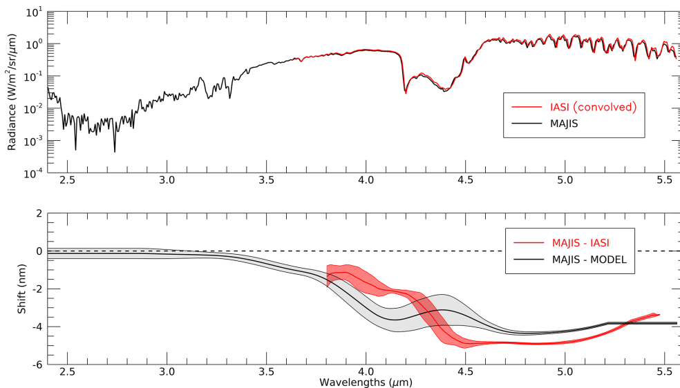
Figure 4. Top panel: Best collocated and concomitant IASI spectrum (red) and MAJIS IR spectrum (black); bottom panel: The spectral residuals between the MAJIS and IASI spectra (presented in the top panel are shown in red with their 1\sigma -uncertainties envelop). The spectral residuals with respect to the 4A/OP radiative transfer model for the same MAJIS pixel (from Fig. 2d) are shown in black with their 1\sigma -uncertainties envelop for comparison.
