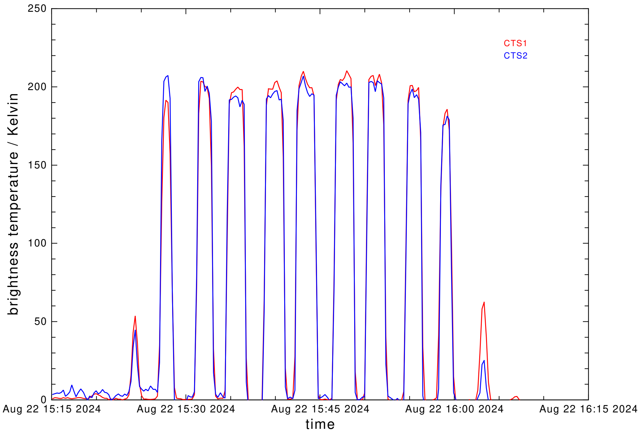
ObsID 00375 - average CTS brightness temperature
