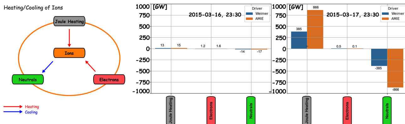
Figure 4. Left: Overview of the main energy sources and energy flow to and from the Ions in the Lower Thermosphere–Ionosphere. Terms in red arrows correspond to heating of the ions whereas terms in blue arrows correspond to cooling of the ions. Right (Middle): Quantification of the main energy terms at the peak of (one day before the peak of) St. Patrick's day storm. Two electric potential drivers are used, according to the models by Weimer 2005 and AMIE, as marked.
