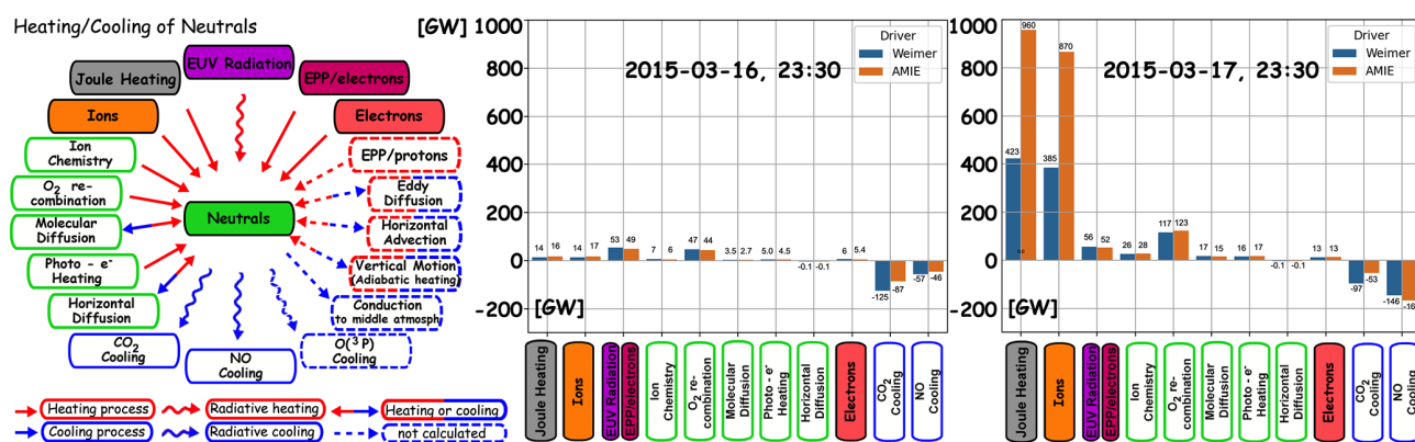
Figure 3. Left: Overview of the main energy sources and energy flow to and from the neutrals in the Lower Thermosphere–Ionosphere. Terms in solid arrows and boxes are estimated through TIE-GCM, whereas terms in dashed arrows and boxes are not calculated. Right (Middle): Quantification of the main energy terms at the peak of (one day before the peak of) St. Patrick’s day storm. Two electric potential drivers are used, according to the Weimer 2005 and the AMIE models, as marked.
