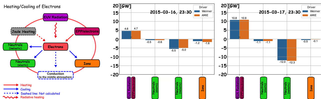
Figure 5. Left: Overview of the main energy sources and energy flow to and from the Electrons in the Lower Thermosphere–Ionosphere. Terms with red arrows correspond to heating of the electrons whereas terms with blue arrows correspond to cooling of the electrons. Right (Middle): Quantification of the main energy terms at the peak of (one day before the peak of) St. Patrick's day storm. Two electric potential drivers are used, according to the models by Weimer, and AMIE, as marked.
