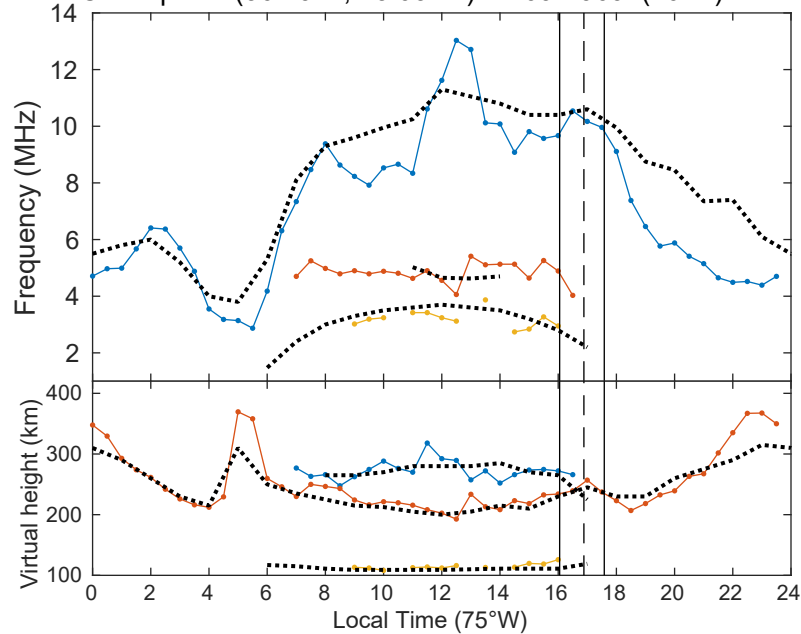
Concepción (36.79°S, 73.03°W) 11-09-1969 (20 %)
