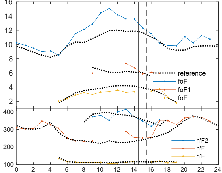
Concepción (36.79°S, 73.03°W) 12-11-1985 (17 %)
