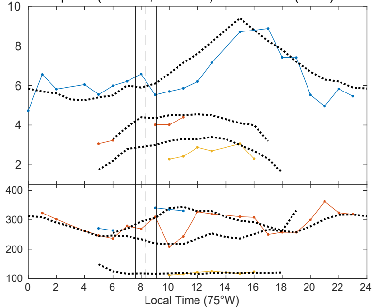
Concepción (36.79°S, 73.03°W) 12-11-1985 (17 %)
