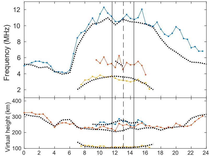
Concepción (36.79°S, 73.03°W) 11-09-1969 (20 %)
