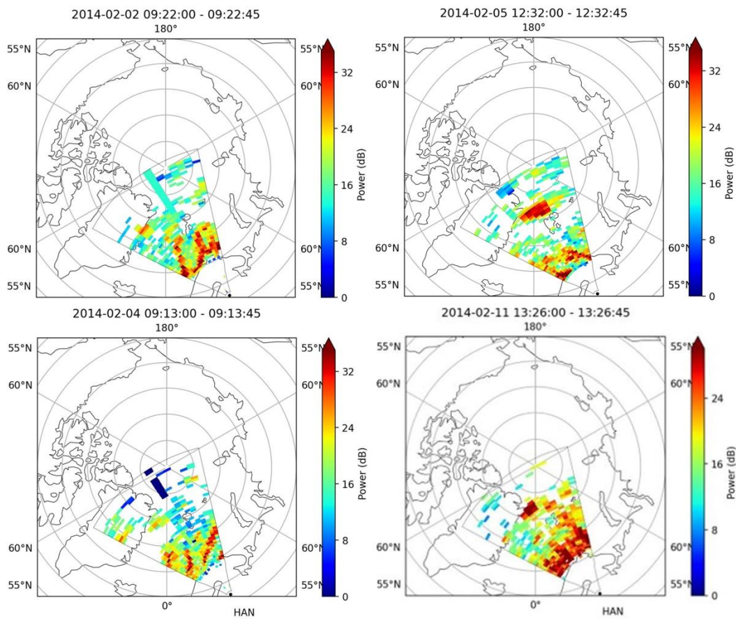
Figure S1. Shows few examples of MSTIDs with different orientations in the Hankasalmi radar FAN plots.
