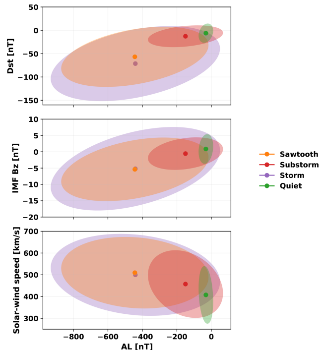
Figure 5. Modes of the magnetosphere with their drivers and responses. (top) Dst, (middle) IMF B_z , and (bottom) solar wind speed as function of the AL index. The solid dots show the mean in each category, with an ellipse created by the standard deviation of the distribution of values around the mean. Quiet time is defined as times where the AL index is greater than -100 nT. Substorms are defined as the time within 3 hours after onsets chosen by Ohtani and Gjerloev (2020). Storms are defined as times within 6 h of Dst peak below -75 nT. Sawtooth intervals include times after the first sawtooth onset in the sequence to the last onset in the sequence.
