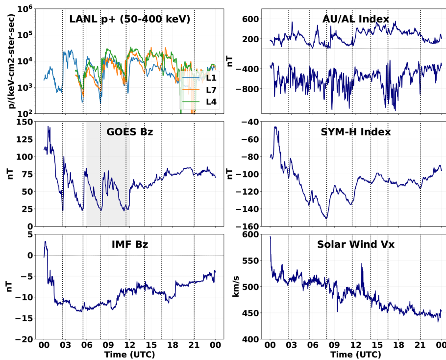
Figure 1. An example of a sawtooth event during 18 April 2002. Left: (top) Geosynchronous orbit ion fluxes from the Los Alamos geostationary satellites the LANL energetic particle instruments. (middle) B_{z,GSM} from GOES-10. (bottom) IMF B_z from the OMNI database. Right: (top) AU/AL Indices, (middle) SYM-H Index, and (bottom) solar wind speed from the OMNI database. The sawtooth onsets are indicated with vertical dashed lines.
