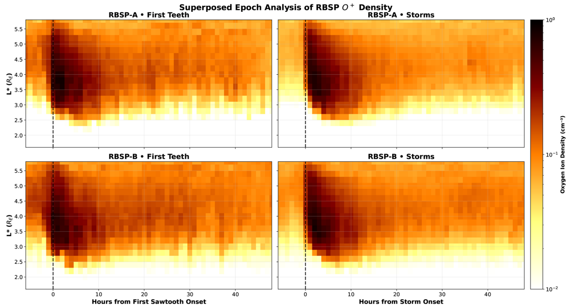
Figure 6. Superposed epoch analysis of RBSP-A and RBSP-B oxygen ion observations from the HOPE instrument. The x -axis represents time relative to epoch time. The observations are sorted into half-orbit bins and sorted relative to their L^* value. The timestamps represent the value at the center of the half-orbit. The oxygen number density is shown color coded in units of \text{cm}^{-3} .
