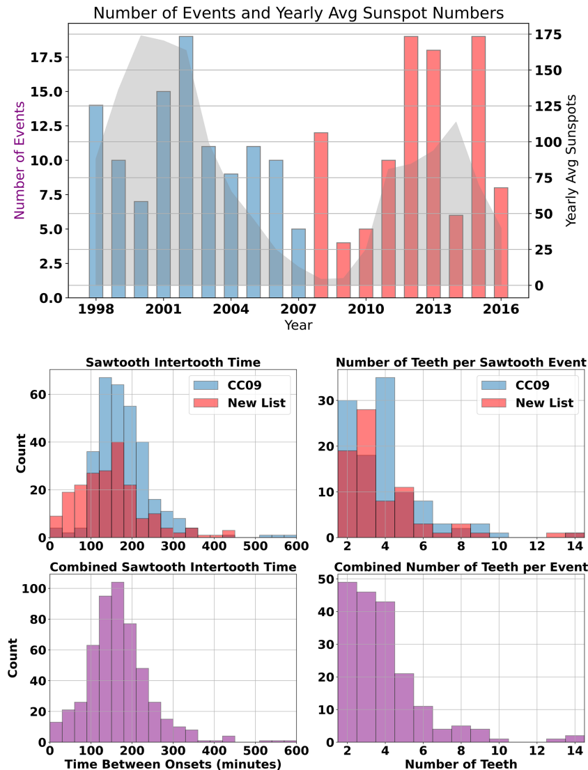
Figure 2. (top) Annual distribution of sawtooth event occurrence with the annual sunspot number on the background. (middle left) Average duration between two sawtooth injection onsets (intertooth interval) for this study (red) and CC09 (blue). (middle right) Average number of teeth per event for this study (red) and CC09 (blue). (bottom left) Combined average duration between sawtooth injections. (bottom right) Combined average number of teeth per event.
