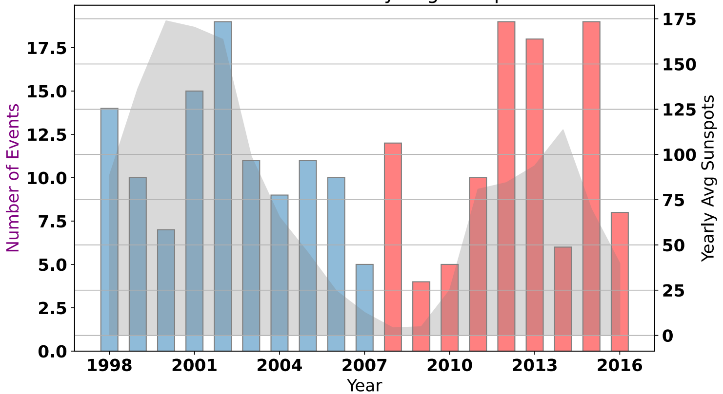
Number of Events and Yearly Avg Sunspot Numbers
