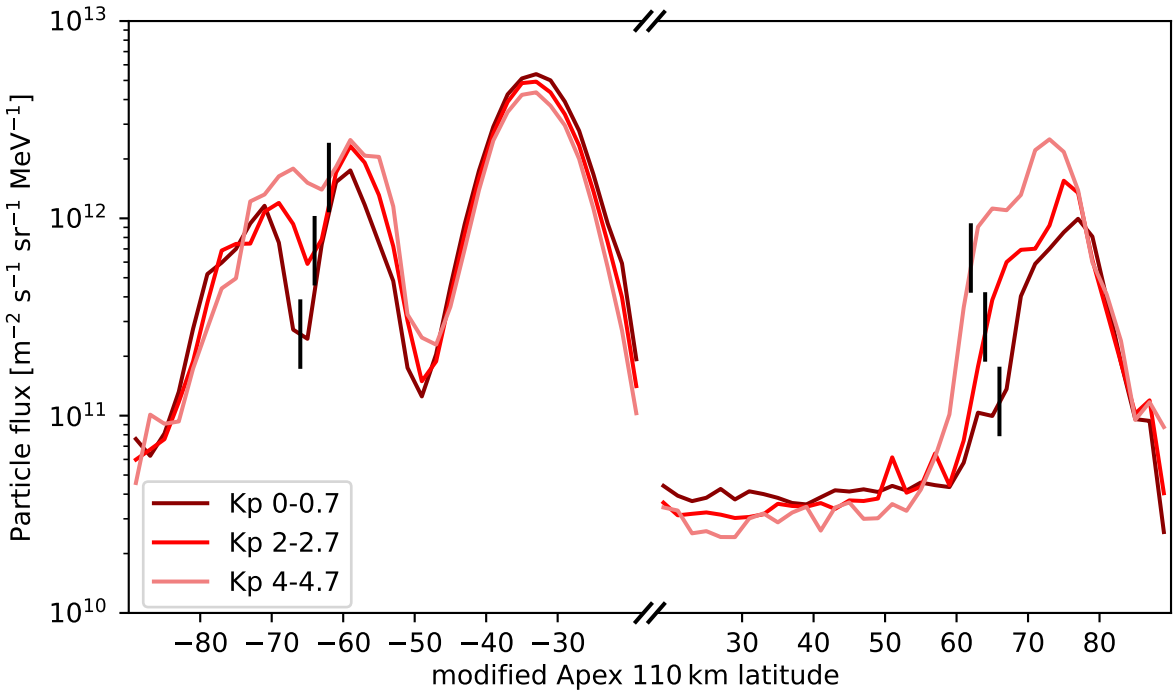
Dependence on geomagnetic disturbance: TED 0° proton band 11
