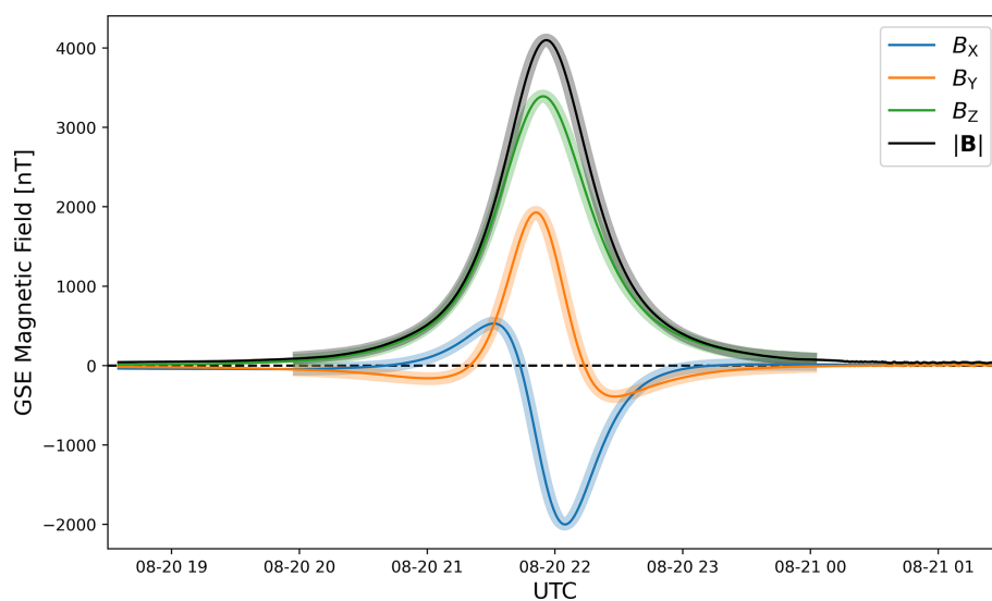
Figure 4. Magnetic field vector measured by J-MAG around Earth closest approach (solid lines), overlaid with model field from IGRF-14 and Tsyanenko 2001 model for the Juice LEGA trajectory (thick, transparent lines), all in GSE coordinate system.
