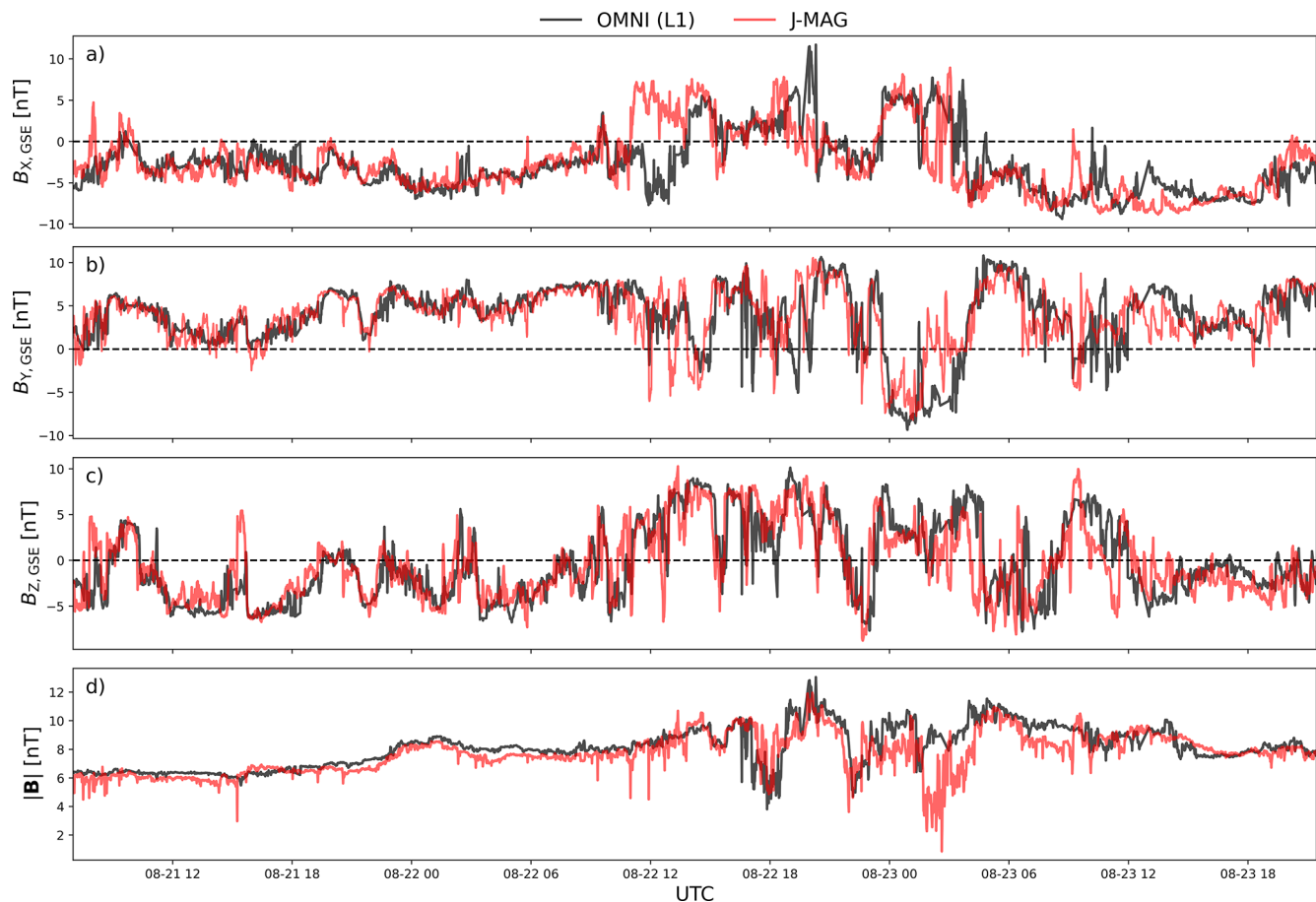
Figure 8. Comparison of J-MAG measurements (red) with those from OMNI (measured at L1 by Wind, grey), over several days in the solar wind after the LEGA. During this time, Juice moved around 120 R_E duskward from Earth. All field vectors shown in GSE coordinate system.
