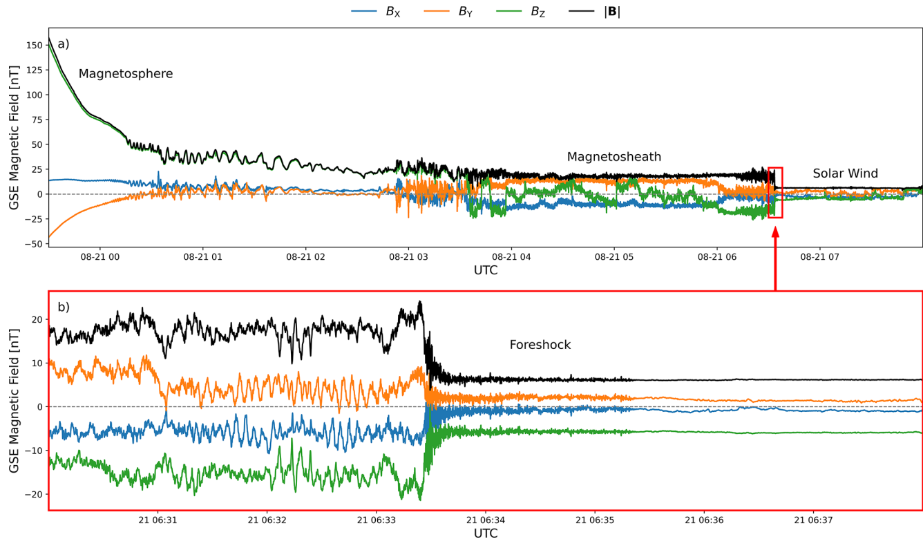
Figure 7. J-MAG magnetic field measurements (GSE) during magnetospheric exit on 21 August. Panel (a) shows the field vector and magnitude as the spacecraft transited the magnetosheath and entered the solar wind. Panel (b) shows a zoom of the bow shock crossing (red square in top panel).
