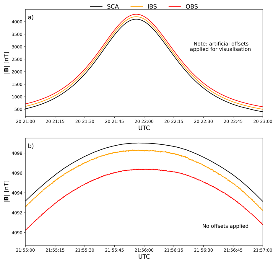
Figure 3. Magnetic field magnitude of the three J-MAG sensors around the Earth closest approach. Panel (a) shows two hours centred on closest approach, with artificial offsets of +100 and +200 nT added to IBS and OBS data, respectively, to aid visualisation at this scale. Panel (b) is a zoom on the peak field at the two minutes of closest approach (with no artificial offsets applied) showing slight differences between sensors. Note the data presented here have undergone only ground-based calibration (i.e. step 1 in Sect. 3).
