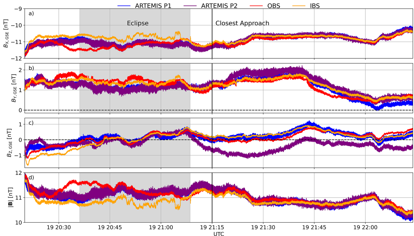
Figure 6. Magnetic field measurements from J-MAG OBS and IBS during the lunar pass, overlaid with observations from the two ARTEMIS probes, all in the GSE coordinate system. Panel (d) shows the field magnitudes. Shaded area indicates the period in which the spacecraft was in an eclipse, and the solid vertical line marks the time of lunar closest approach.
