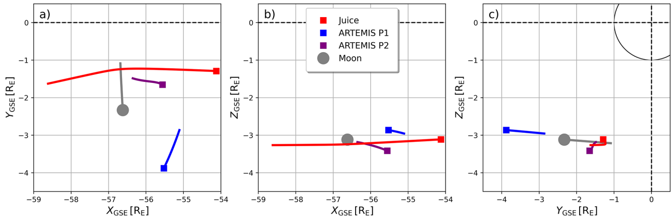
Figure 5. Orbital trajectories of Juice, the two ARTEMIS probes, and the Moon during the lunar pass, 19 August 20:20–22:30. All positions in Earth radii, GSE coordinate system, shown in all three planes. Final positions of the bodies in this period indicated with markers.
