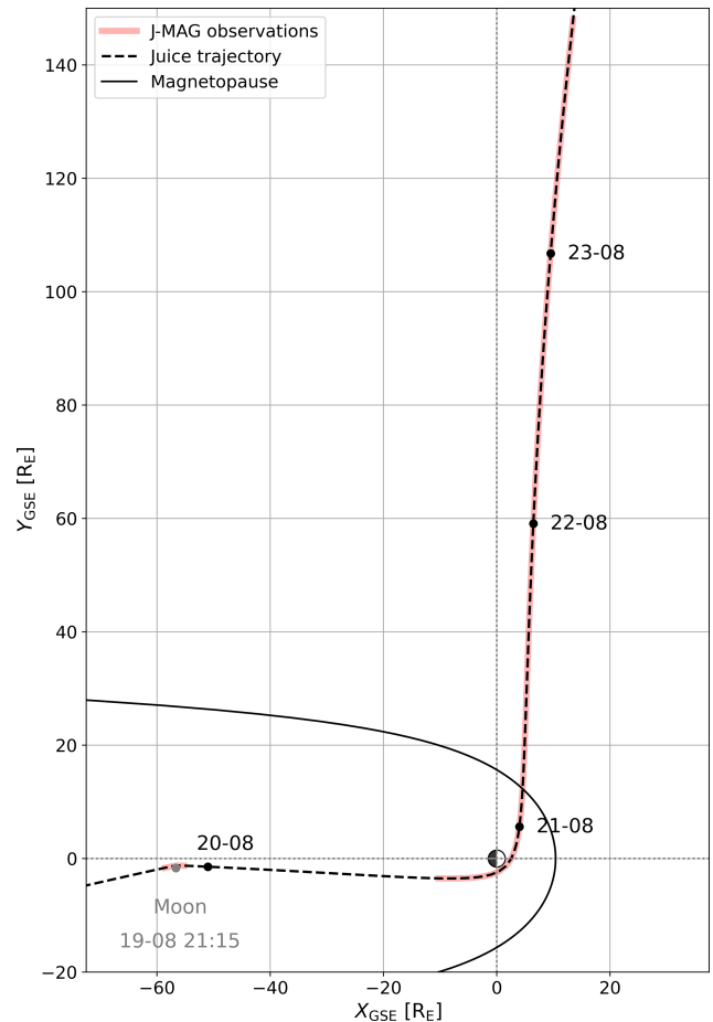
Figure 1. Orbital trajectory of Juice spacecraft during the LEGA, shown in the GSE X – Y plane, in units of Earth radii. Dashed black line shows spacecraft path, with the position at midnight of each day marked with a black dot. The portions of the flyby for which J-MAG was recording science data are highlighted in red. Solid black line shows an approximate position of the magnetopause as predicted by the Shue et al. (1998) empirical model, parametrised with average solar wind conditions during the LEGA period. The position of the Moon at lunar closest approach is also marked.
