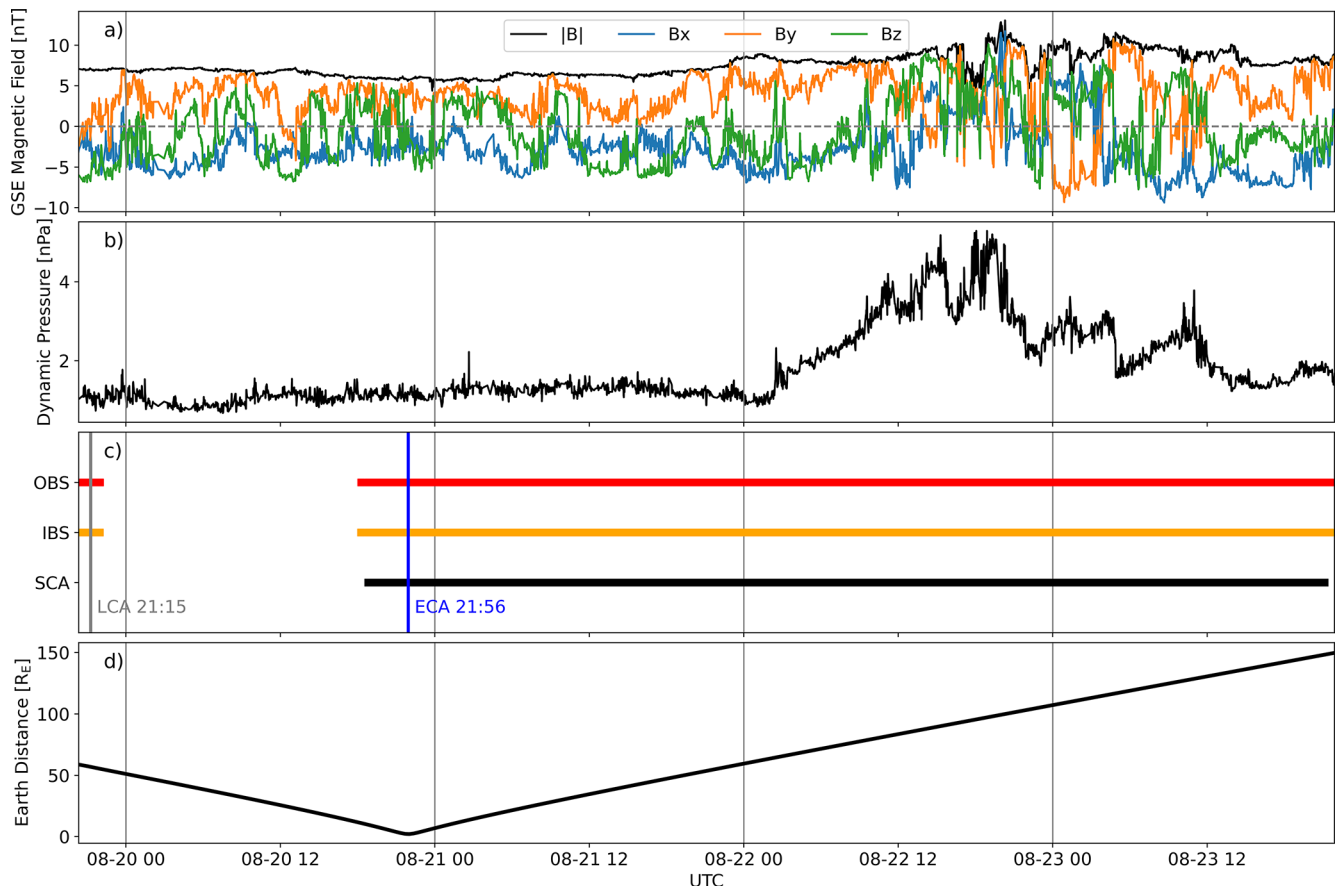
Figure 2. Flyby context and timeline. Panel (a) shows the interplanetary magnetic field (GSE) from the OMNI database, that is, measured at L1 and algorithmically propagated to Earth's bow shock. Panel (b) shows the solar wind dynamic pressure during the flyby period. Panel (c) shows a timeline of J-MAG sensor operation, with the lunar closest approach (LCA) and Earth closest approach (ECA) marked. Panel (d) shows the distance of Juice from Earth.
