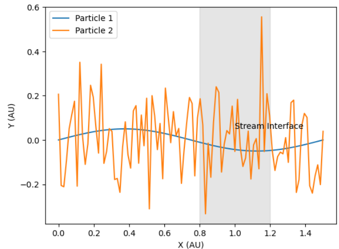
Figure 6. Plots of two modelled particle trajectories: particle 1 is with low scattering that travels directly through the stream interface, and particle 2 is with high scattering that has a random-walk trajectory, indicating increased pitch angle changes.
