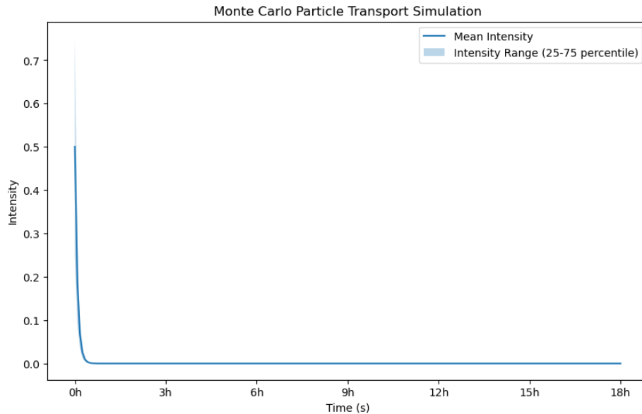
Figure 4. The modelled intensity profile shows the mean value over an ensemble of stochastic trajectories including microburst scattering. The percentile bands highlight the variability.
