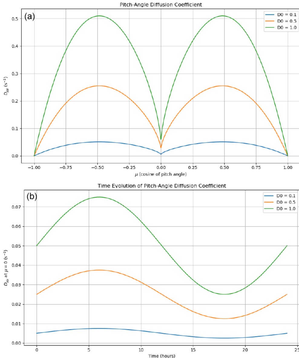
Figure 8. Pitch angle diffusion coefficient ( D_{\mu\mu} ) characteristics. (a) D_{\mu\mu} as a function of \mu (cosine of pitch angle) for different D_0 values. (b) Time evolution of D_{\mu\mu} at \mu = 0 over 24 h, simulating passage through a stream interaction region. The model uses D_{\mu\mu}(\mu, t) = D_0(t)(1 - \mu^2)(|\mu|^{5/3-1} + 0.05) , where D_0(t) = D_0(1 + 0.5 \sin(2\pi t/24)) represents time-dependent scattering conditions.
