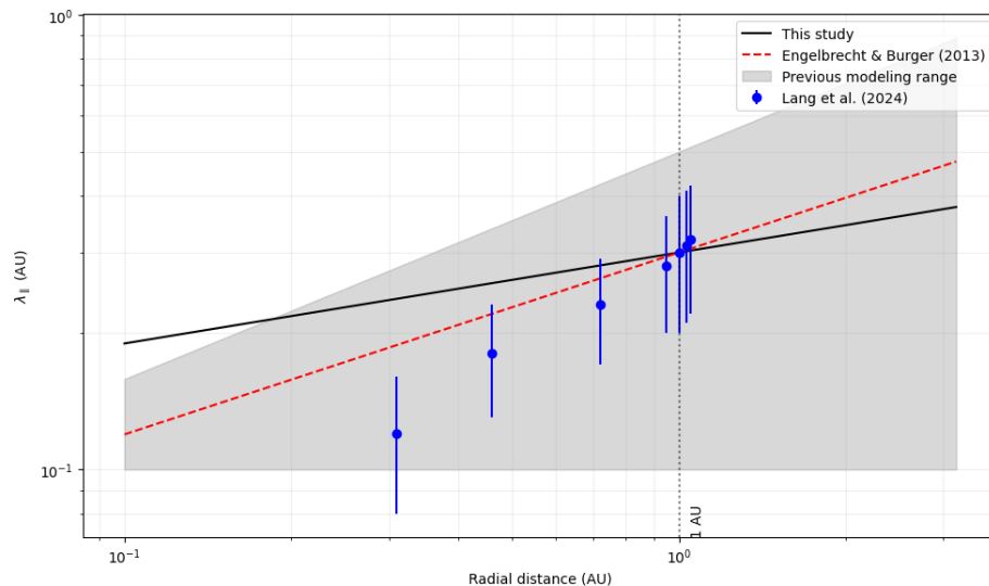
Figure 10. Radial dependence of the parallel mean free path ( \lambda_{\parallel} ) for GeV protons. The solid black line represents our model ( \lambda_{\parallel} = 0.3(r/1 \text{ AU})^{0.2} \text{ AU} ). The dashed red line shows the theoretical prediction from Engelbrecht and Burger (2013). Blue dots with error bars represent observational data from Lang et al. (2024). The shaded grey area indicates the range of \lambda_{\parallel} values used in previous modelling efforts based on Dröge et al. (2010) and He et al. (2011). The vertical dotted line marks 1 AU for reference.
