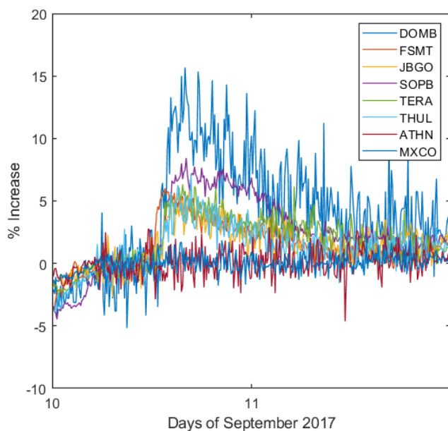
Figure 2. NM observation of GLE 72 from the selected stations used in this study.
