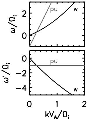
(b) pickup ion scenario
