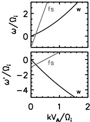
(a) foreshock ion scenario
