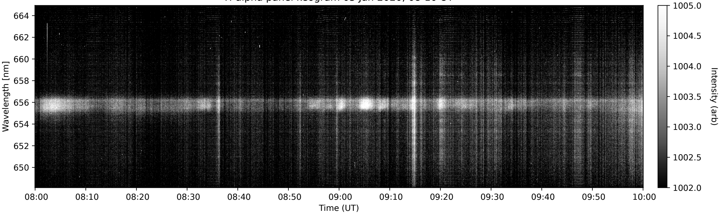
H-alpha panel keogram 03 Jan 2020, 08-10 UT
