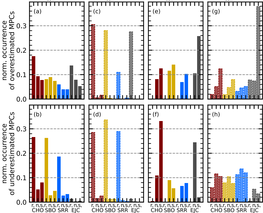
SH98 deviations with \theta_{B,n} < 45^\circ
