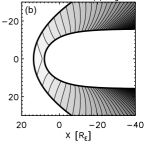
Radial mapping
