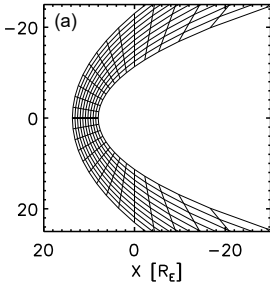
Parabolic boundaries
