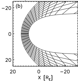
Non-parabolic boundaries
