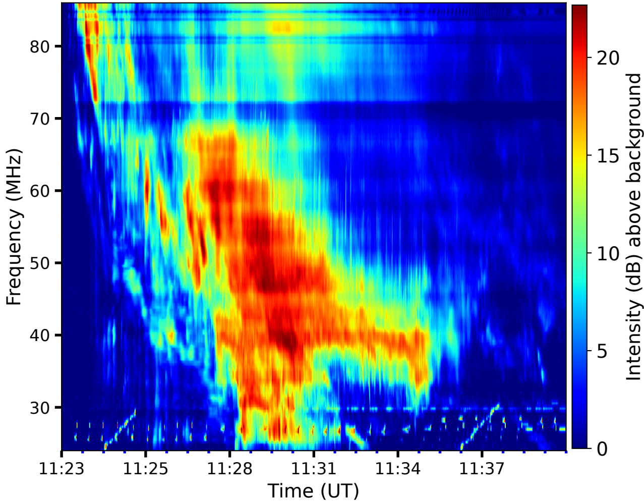
2022/03/28 Radio flux density, e-CALLISTO (Arecibo-Observatory)
