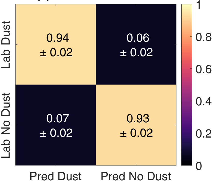
(c) The SVM Classifier
