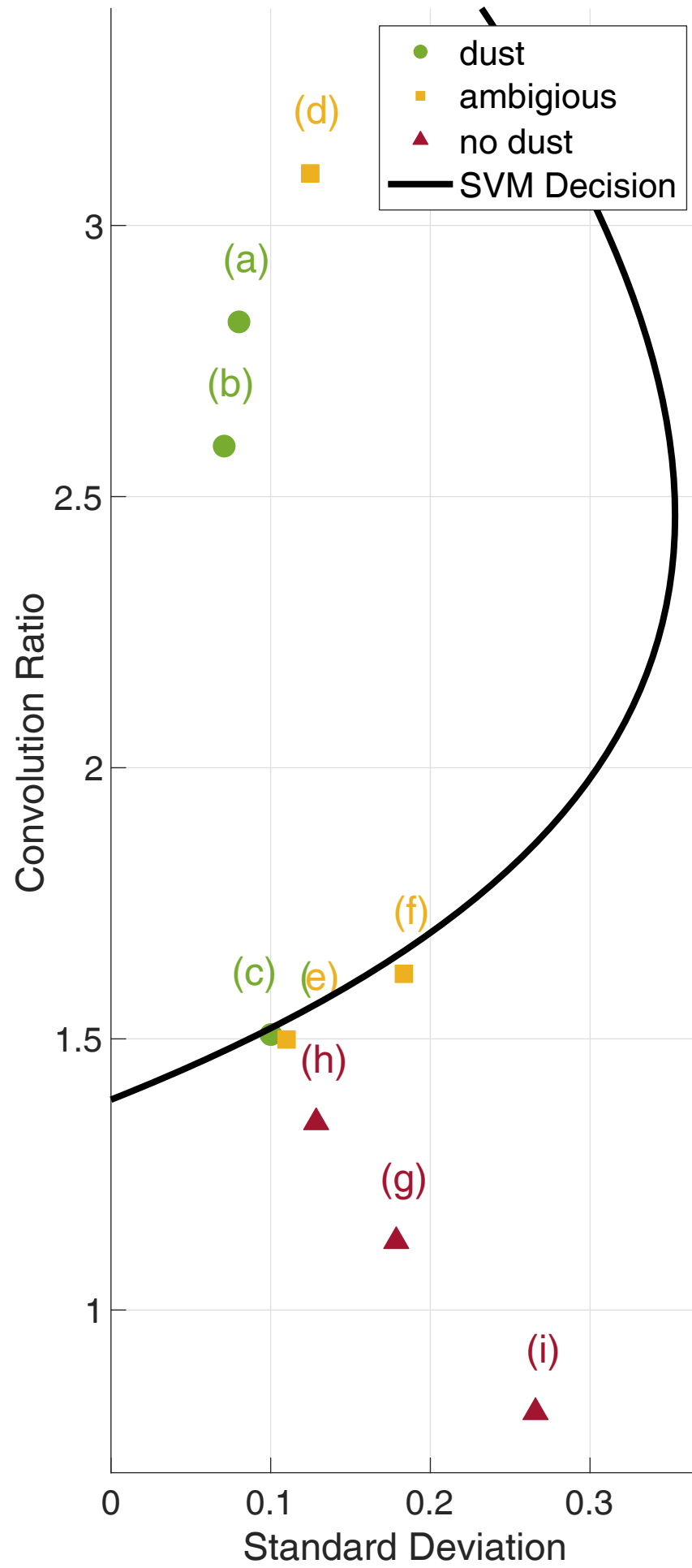
(j) SVM Classification
